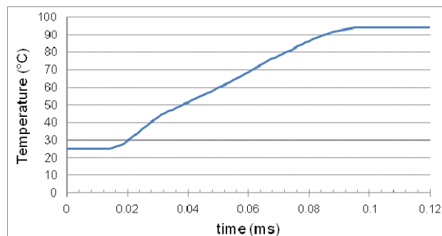
Figure 8: History of temperature distribution in the specimen during the compression process at point A (see Fig. 3).
