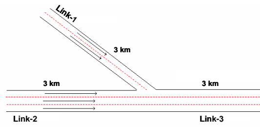
Figure 1: Motorway merge road geometry
