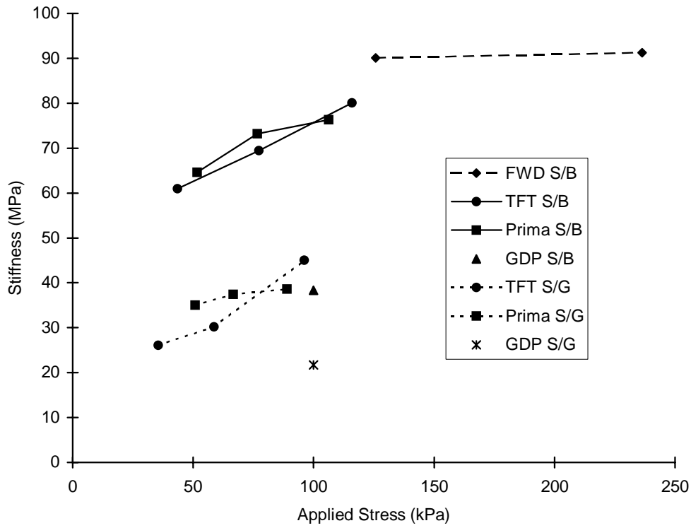
Figure 3. Relationship between Stiffness and Applied Stress for the FWD, TFT, Prima 100 and GDP on Sub-Base (S/B) and Subgrade (S/G) at a Controlled Trial Construction Site (400mm Capping and 150mm Sub-Base over a Clay Subgrade)
