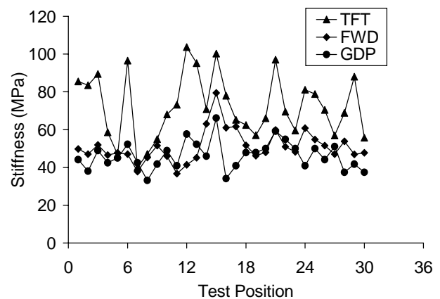
Figure 2. Variability of Stiffness along a 36m Test Length at the M65 (Contract 1) (350mm Capping Over a Soft Clay Embankment)
