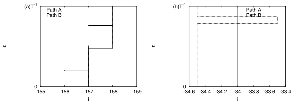
Figure 10. Example path configurations on (a) the rectangular ladder and (b) the staggered ladder. Hopping events on different paths on the rectangular ladder are very correlated in time. On the staggered ladder, there are two degenerate configurations, and paths are just as likely to sit on either of the two neighbouring sites, significantly reducing the correlation between kinks. ( \omega/t = \lambda = 4 in both cases.)
