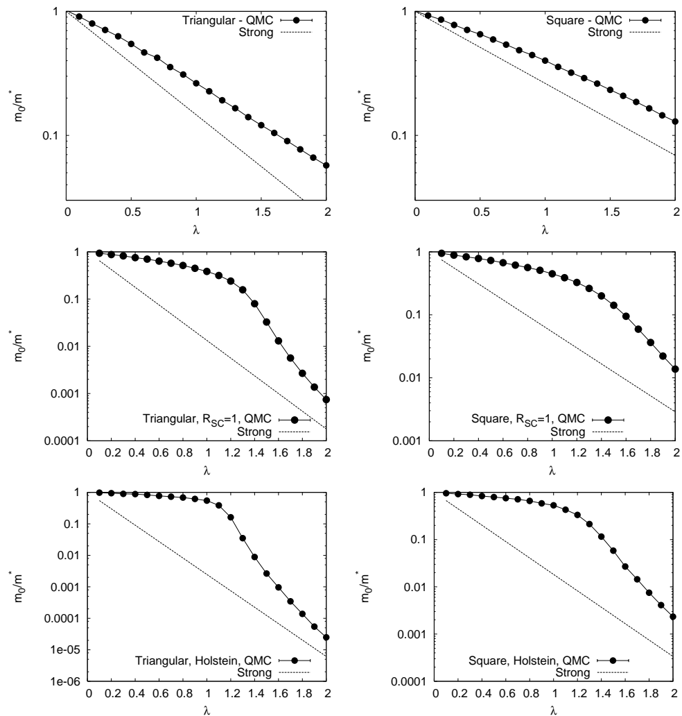
Figure 4. Inverse effective mass of the discrete Fröhlich polaron on square and triangular lattices. \omega/t = 1 , and \lambda is varied. Triangular lattices are shown on the left, and square lattices are shown on the right. From top to bottom, the screening radius of the interaction is decreased, with the top graphs showing Fröhlich interaction R_{sc} \rightarrow \infty , middle graphs screened interaction R_{sc} = 1 and the bottom graphs the Holstein interaction R_{sc} = 0 . Fröhlich polarons are significantly lighter than their Holstein counterparts because the long range interaction leads to pre-distortions of the lattice before a hopping.
