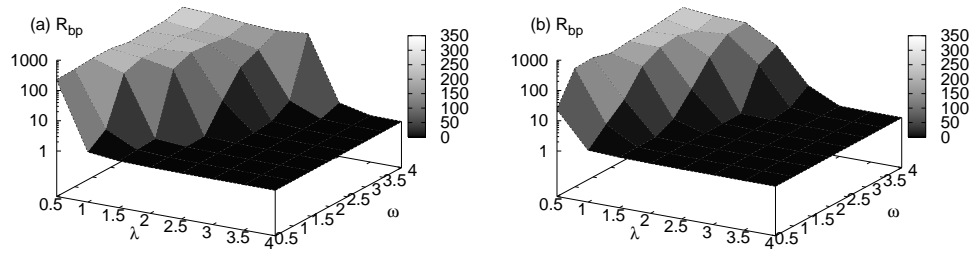
Figure 7. Size of the bipolaron for (a) the rectangular ladder and (b) the staggered ladder. Not only is the bipolaron on the staggered ladder lighter than that on the rectangular ladder, its size is also smaller for equivalent \lambda .
