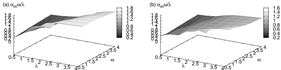
Figure 9. Mass isotope exponent of the bipolaron for (a) the rectangular ladder and (b) the staggered ladder. Again, we can see that the strong coupling limit is achieved at significantly lower \lambda on the staggered ladder. The isotope exponent is also smaller on the staggered ladder, demonstrating a much smaller range of mass from weak to strong coupling.
