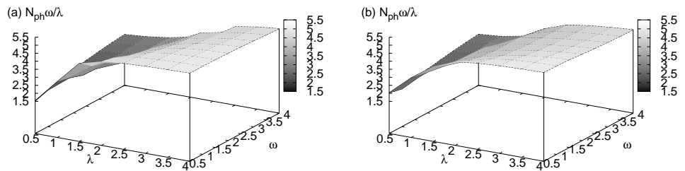
Figure 8. Number of phonons associated with the bipolaron for (a) the rectangular ladder and (b) the staggered ladder, weighted by phonon frequency and electron phonon coupling. Again, we can see that the strong coupling limit is achieved at significantly lower \lambda on the staggered ladder. It is interesting to note that the states with large \omega have a smaller number of phonons. This is consistent with the anti-adiabatic approximation: When phonon frequency is large, creating phonons becomes difficult, and phonon wavefunction is the vacuum state. Then the phonon problem maps onto a UV model (discussed later).
