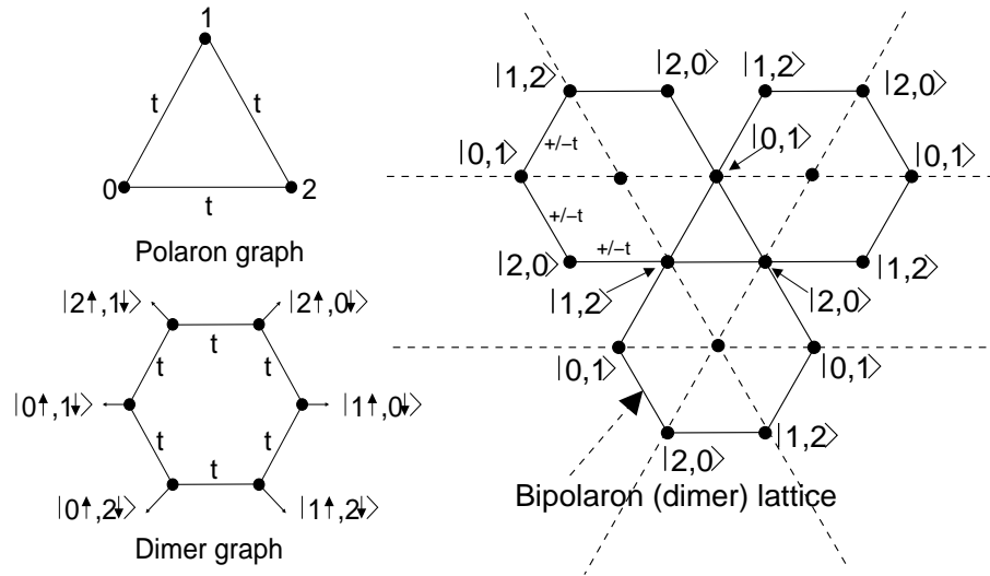
Figure 11. The triangular lattice (thin lines) with a dimer state (circle) at the midpoint of each bond. The polaron and bipolaron states are indicated on one triangle, with spin indices suppressed. The dimer lattice (thick lines) is a kagome lattice.
