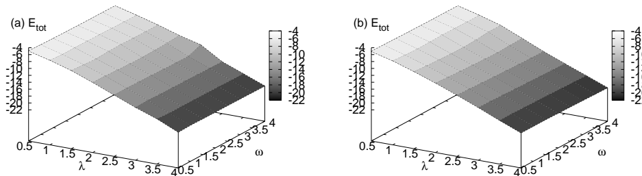
Figure 5. Total energy of the bipolaron for (a) the rectangular ladder and (b) the staggered ladder. A slight change in gradient between weak and strong coupling is just discernable, demonstrating (as we shall see in the coming figures) that the staggered ladder reaches the strong coupling limit at significantly lower \lambda than the rectangular ladder.
