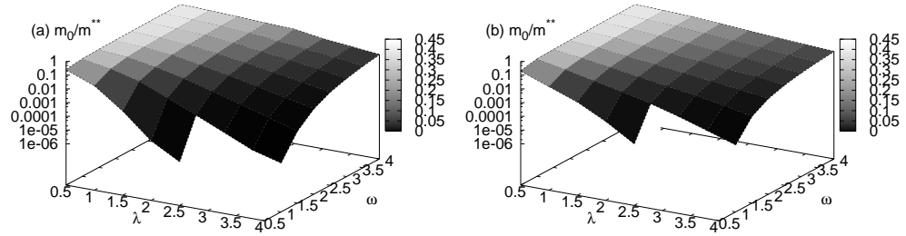
Figure 6. Inverse mass of the bipolaron for (a) the rectangular ladder and (b) the staggered ladder. There is more than an order of magnitude difference between the mass of the bipolaron on the staggered ladder, and that on the rectangular ladder over significant regions of the parameter space. Bipolaron masses on the staggered ladder have recently been shown to have a value commensurate with the polaron mass.
