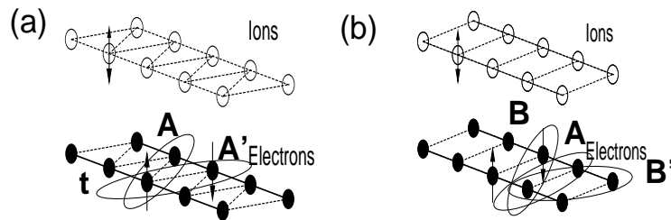
Figure 1. (a) Staggered vs (b) rectangular ladders. Ions are placed one lattice spacing above a ladder of electrons, with one ion per site. The ions are permitted to vibrate in the z -direction only. Electrons inhabit one leg each, with no hopping between the legs. In the strong coupling limit, there are significant geometrical differences. On the staggered ladder, two degenerate near neighbour pairs (A and A') can form, which allows the polaron to scuttle in a crab-like manner with mass proportional to the polaron hopping. Alternatively, on the rectangular ladder there is one near-neighbour state, and in order to move, the pair must break to state A in order to change configuration from state B to B'. Such a state propagates by waddling awkwardly, and has mass proportional to polaron hopping squared.
