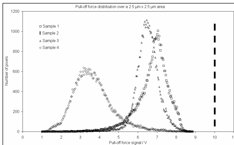
Figure 15a – To show the pull-off force distributions for clean nickel, Dynasylan F8261, Frekote B15/710 NC and Zyvox Waterworks treated release coatings
