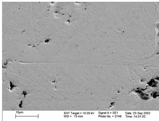
Figure 4a - SEM image of hand polished nickel tooling
