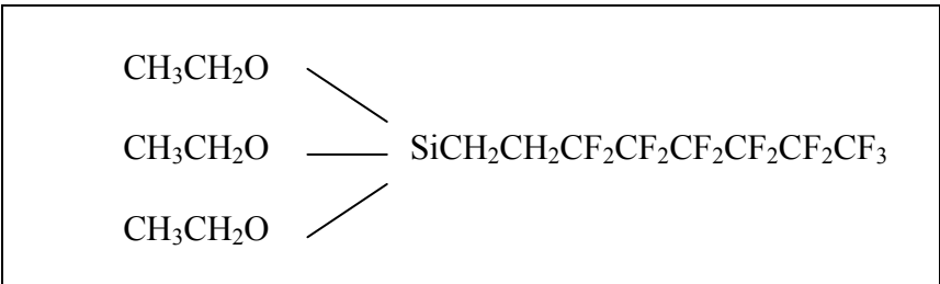
Figure 1 – To show the molecular structure of Dynasylan F8261.
