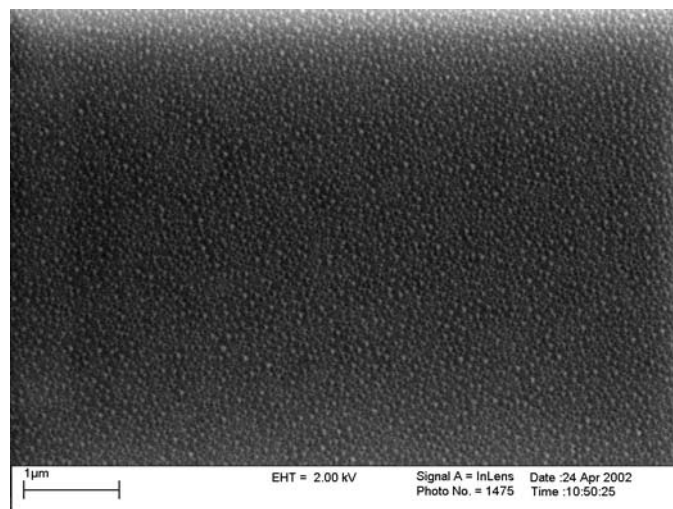
Figure 9a – Low resolution FEGSEM image of fluoroalkylsilane coating on nickel
