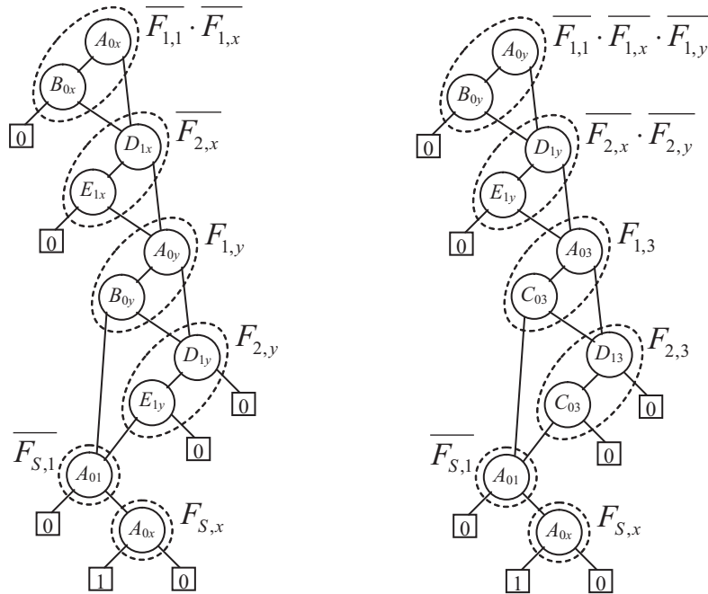
Fig. 10 The BDDs representing the numerators of equations (28) (left) and (29) (right)
