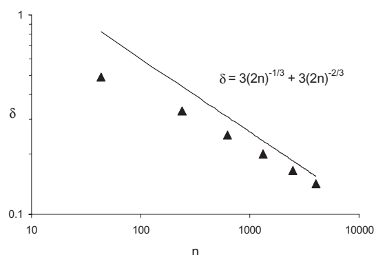
Figure 7. Log-log plot of bounds for \delta_n .
