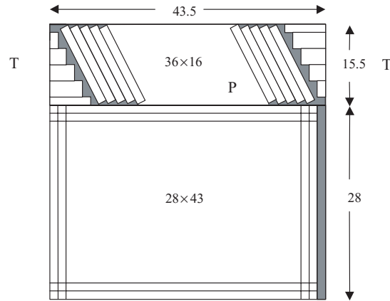
Figure 6. Construction demonstrating s(43^2 + 1) < 43 + \frac{1}{2} .
