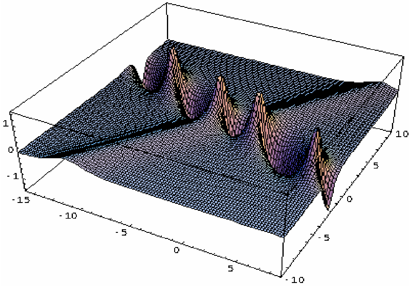
Figure 3a. Interaction between a breather and a positive soliton for \alpha = 6 and \delta = 1
