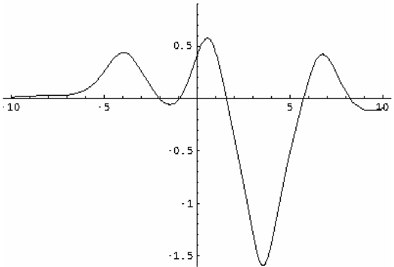
Figure 3d. Interaction between a breather and a positive soliton at t = -1 with \alpha = 6 and \delta = 1
