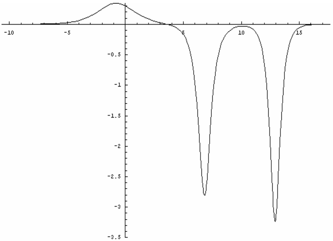
Figure 1f. Interaction among three solitons at t = 2.6s with \alpha = 6 and \delta = 1
