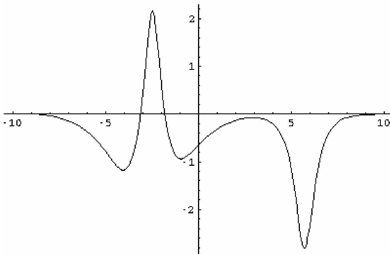
Figure 2g. Interaction between a breather and a negative soliton at t = 2 with \alpha = 6 and \delta = 1
