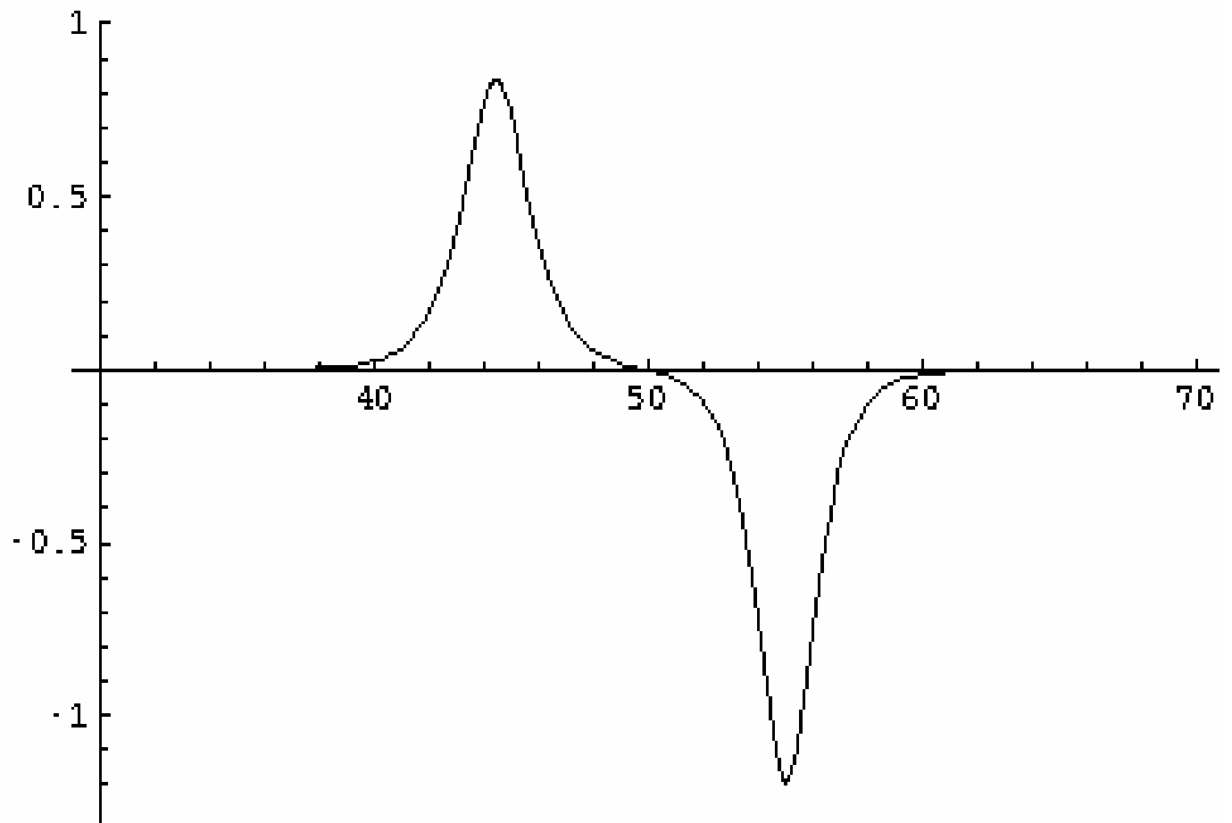
Figure 4c. Motion of a double pole solution at t = 50 with \alpha = 6 and \delta = 1
