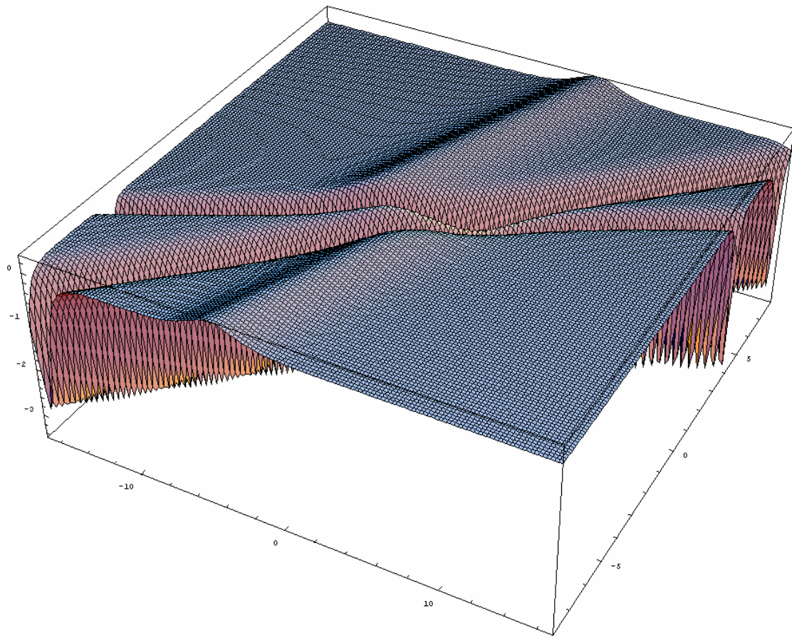
Figure 1a. Interaction among three solitons for \alpha = 6 and \delta = 1
