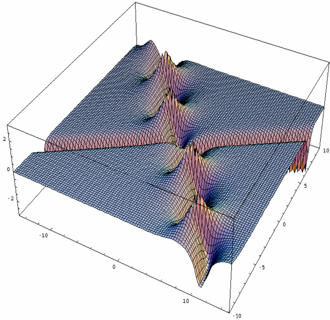
Figure 2a. Interaction between a breather and a negative soliton for \alpha = 6 and \delta = 1
