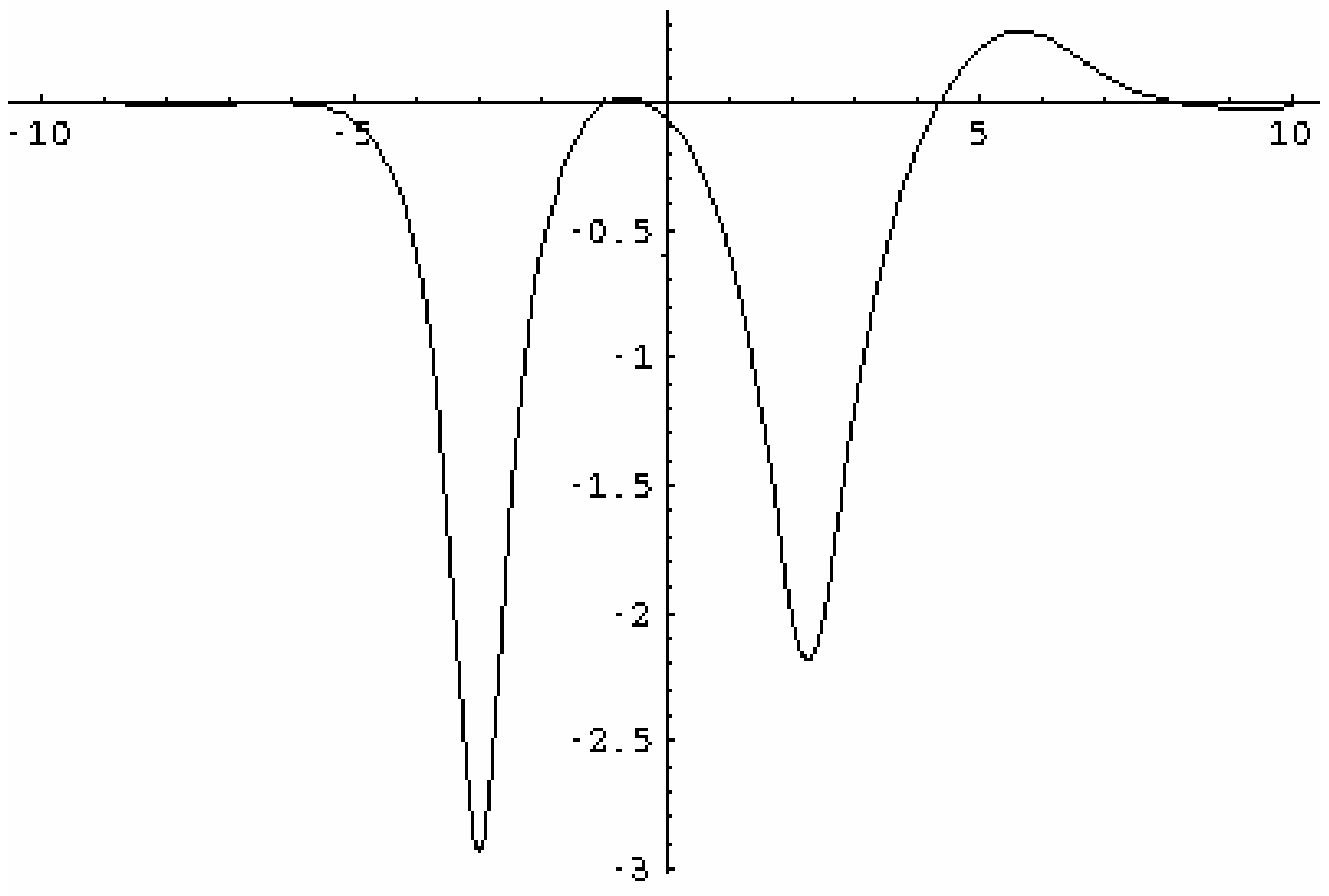
Figure 2d. Interaction between a breather and a negative soliton at t = -1 with \alpha = 6 and \delta = 1
