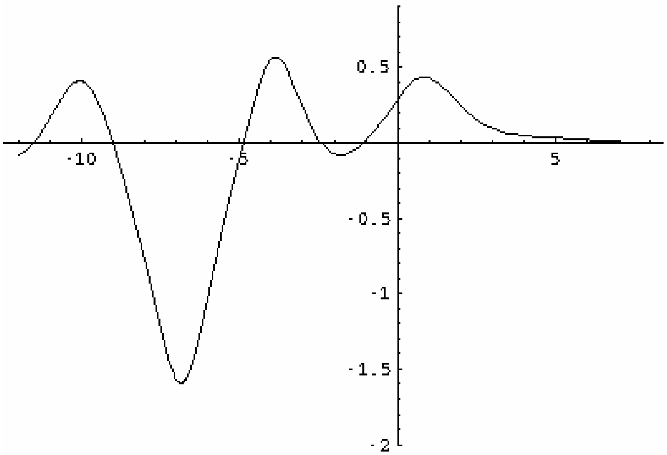
Figure 3g. Interaction between a breather and a positive soliton at t = 2 with \alpha = 6 and \delta = 1
