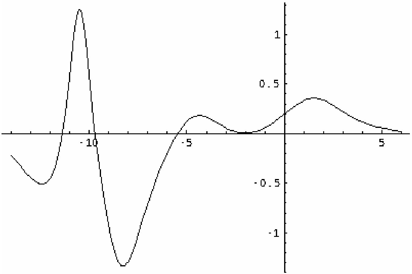
Figure 3h. Interaction between a breather and a positive soliton at t = 3 with \alpha = 6 and \delta = 1
