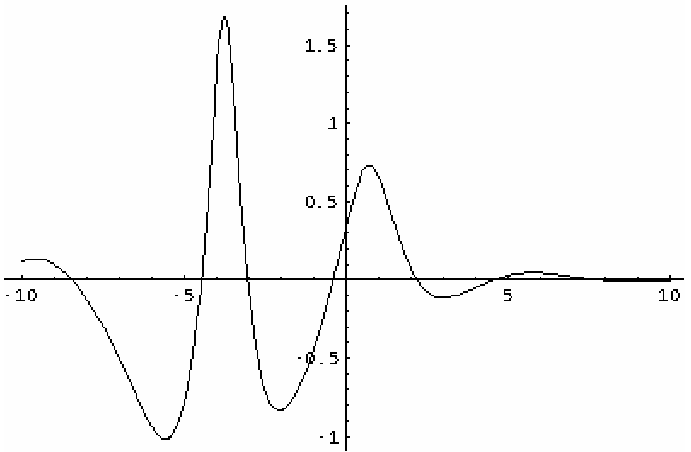
Figure 3f. Interaction between a breather and a positive soliton at t = 1 with \alpha = 6 and \delta = 1
