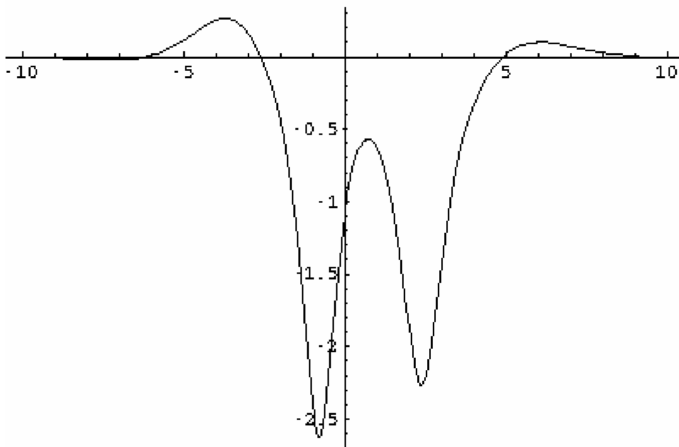
Figure 2e. Interaction between a breather and a negative soliton at t = 0 with \alpha = 6 and \delta = 1
