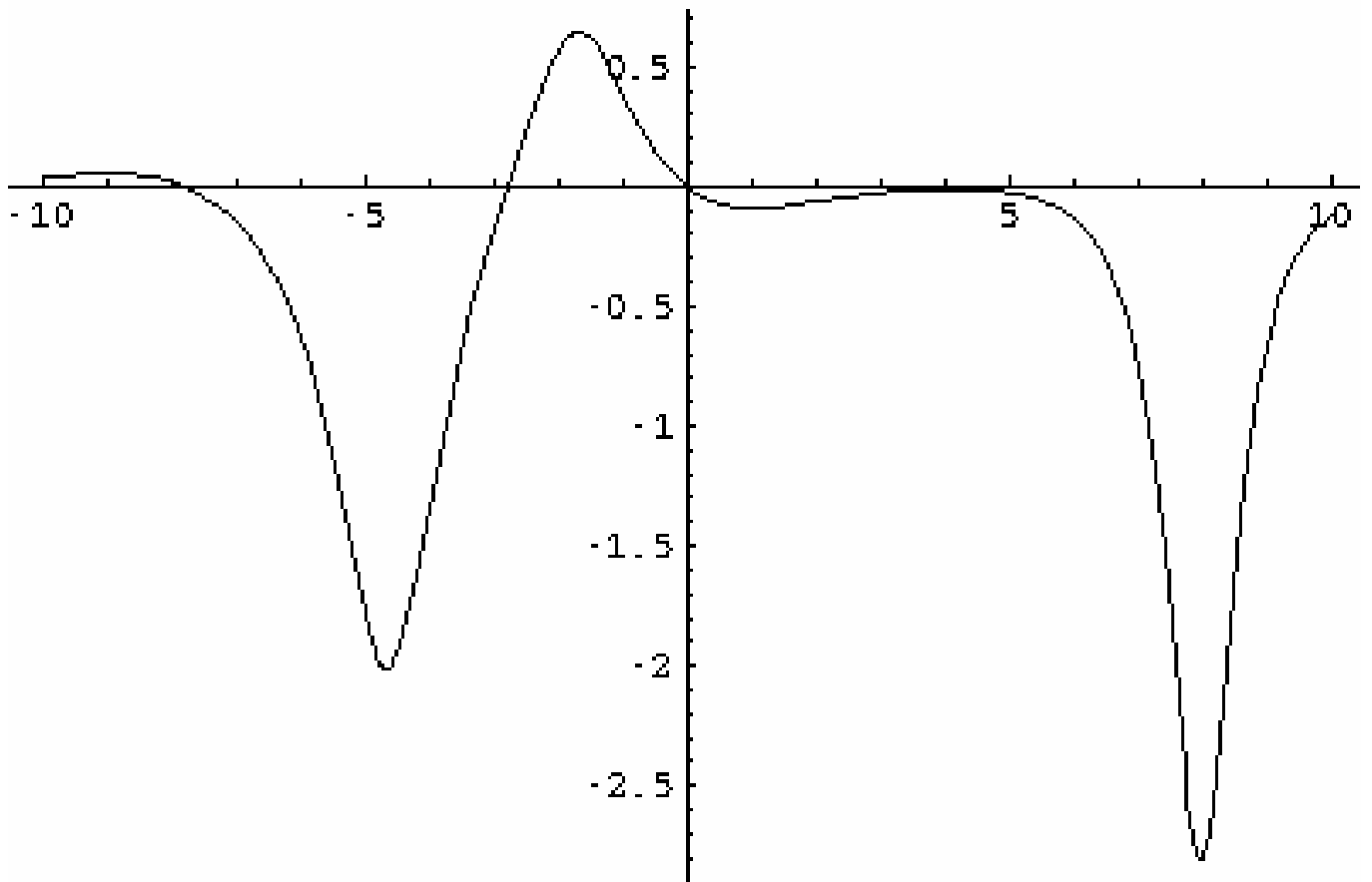
Figure 2h. Interaction between a breather and a negative soliton at t = 3 with \alpha = 6 and \delta = 1
