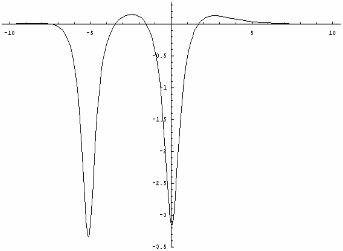
Figure 1c. Interaction among three solitons at t = -1.2 s with \alpha = 6 and \delta = 1
