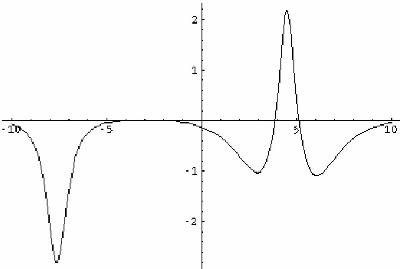
Figure 2b. Interaction between a breather and a negative soliton at t = -3 with \alpha = 6 and \delta = 1
