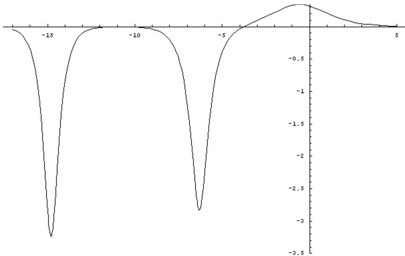
Figure 1b. Interaction among three solitons at t = -3.6s with \alpha = 6 and \delta = 1
