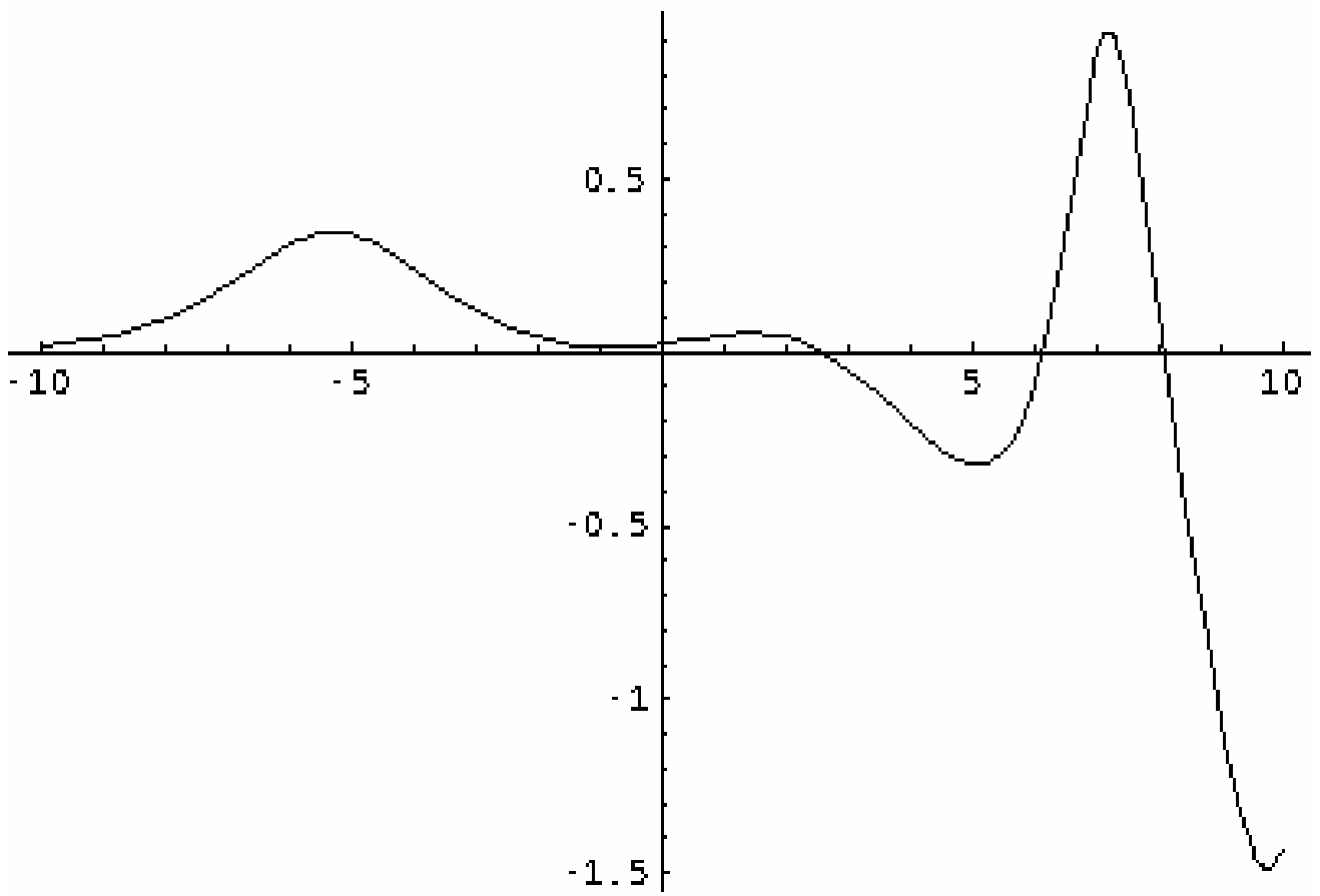
Figure 3b. Interaction between a breather and a positive soliton at t = -3 with \alpha = 6 and \delta = 1
