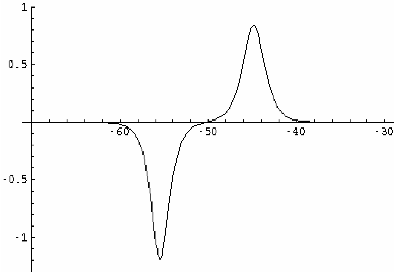
Figure 4a. Motion of a double pole solution at t = -50 with \alpha = 6 and \delta = 1
