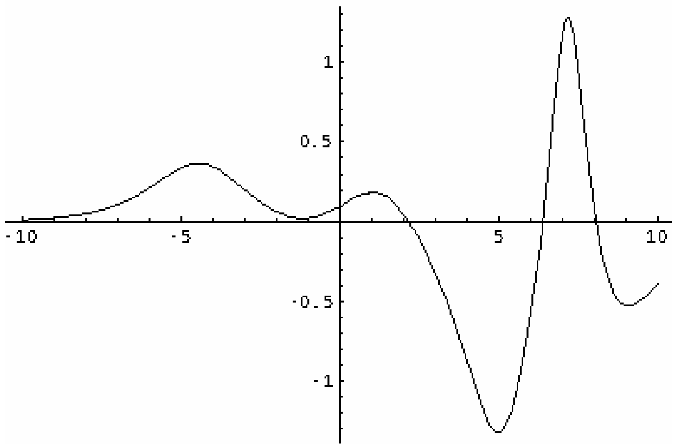
Figure 3c. Interaction between a breather and a positive soliton at t = -2 with \alpha = 6 and \delta = 1
