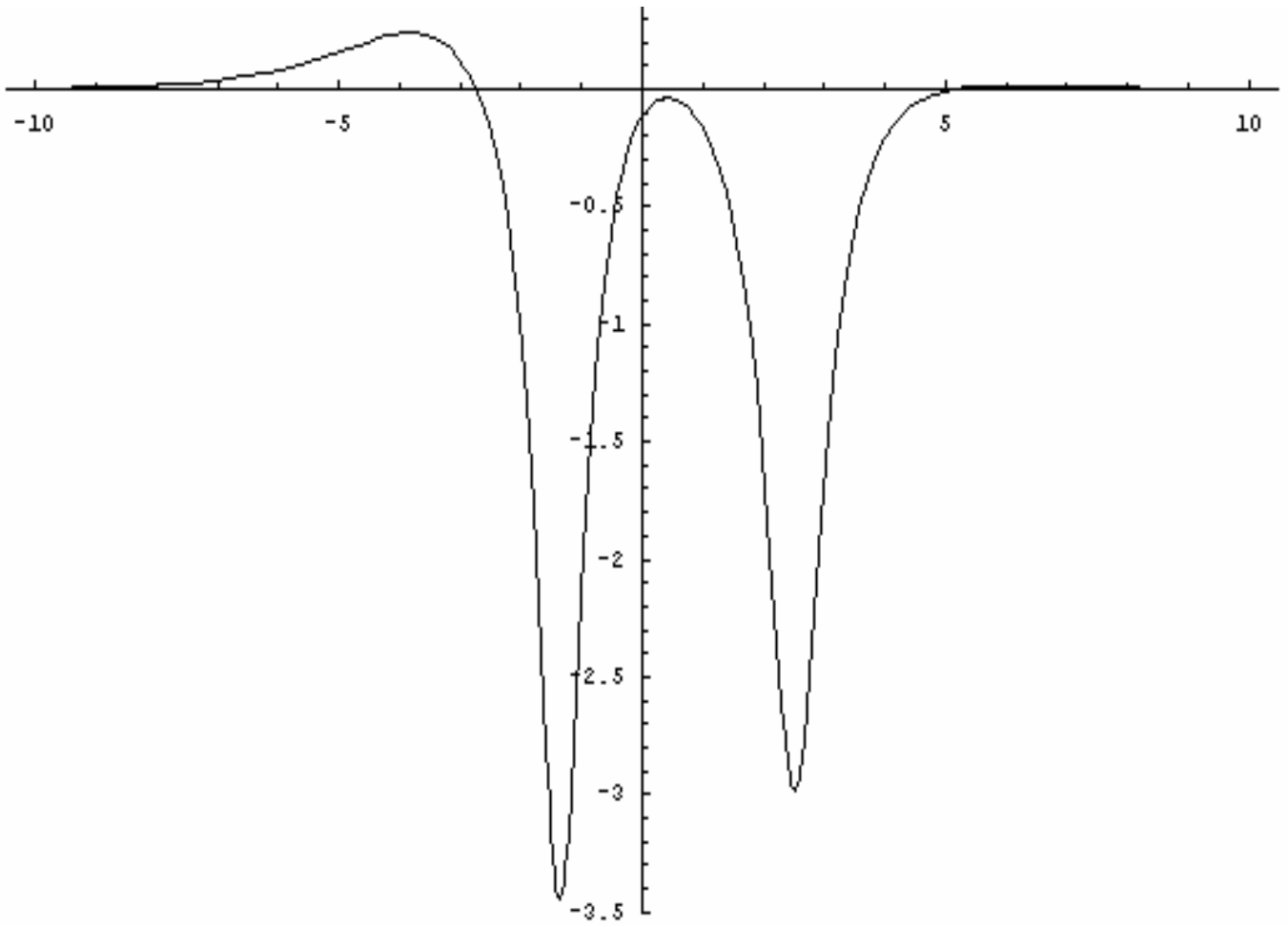
Figure 1d. Interaction among three solitons at t = -0.35s with \alpha = 6 and \delta = 1
