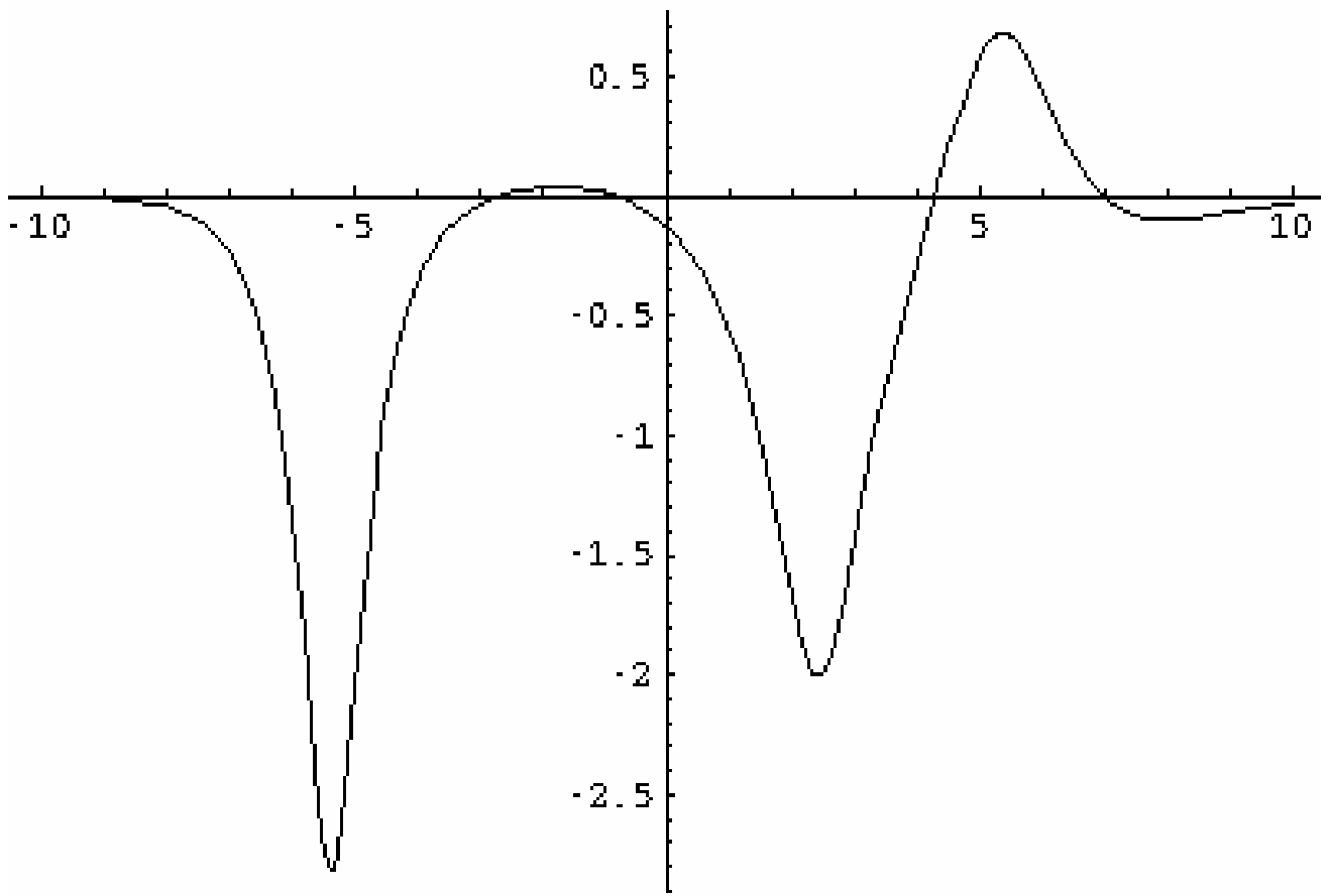
Figure 2c. Interaction between a breather and a negative soliton at t = -2 with \alpha = 6 and \delta = 1
