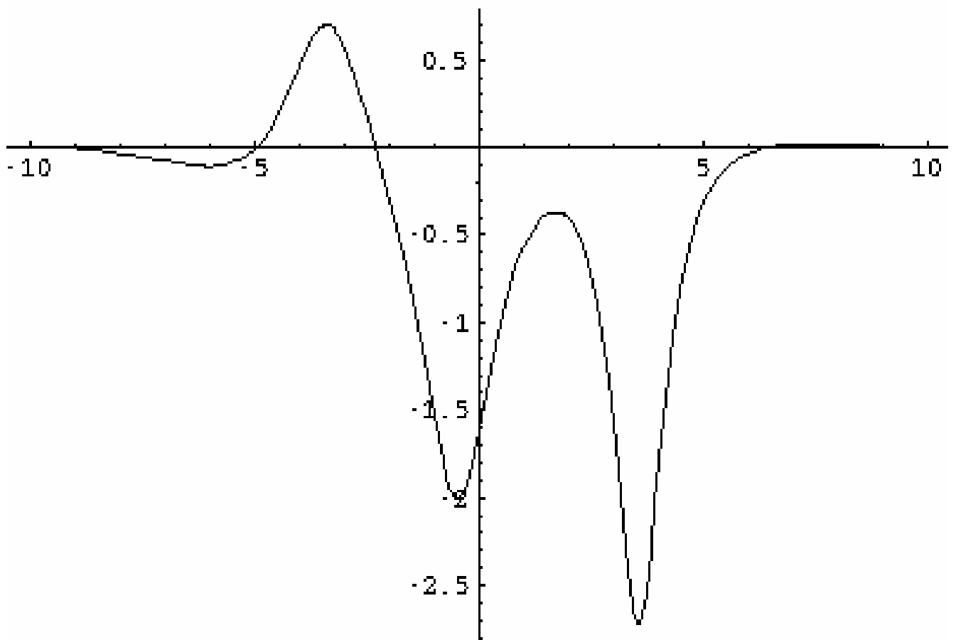
Figure 2f. Interaction between a breather and a negative soliton at t = 1 with \alpha = 6 and \delta = 1
