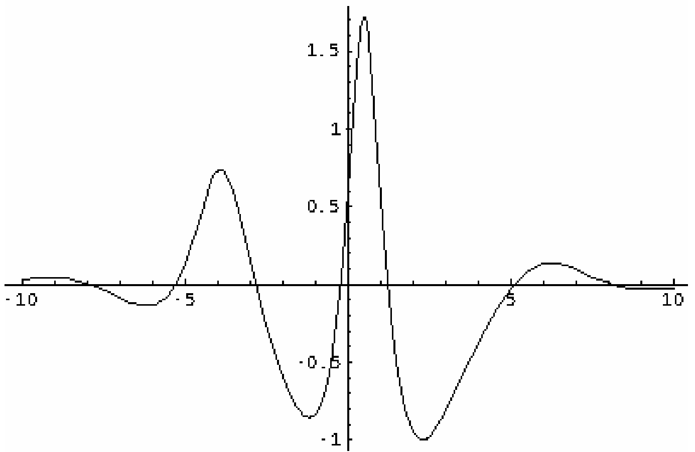
Figure 3e. Interaction between a breather and a positive soliton at t = 0 with \alpha = 6 and \delta = 1
