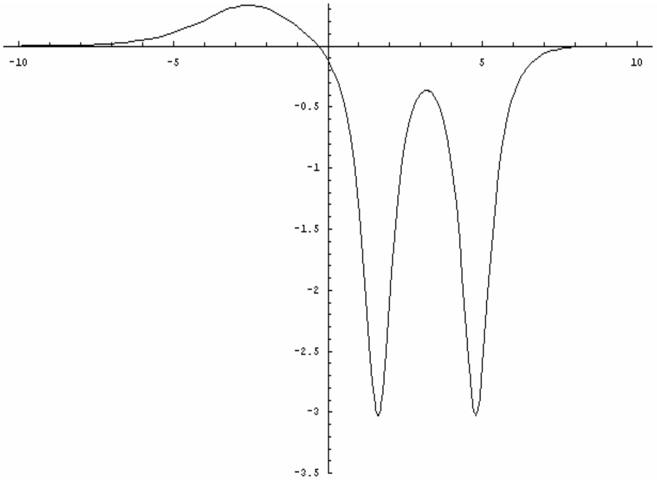
Figure 1e. Interaction among three solitons at t = 0.45s with \alpha = 6 and \delta = 1
