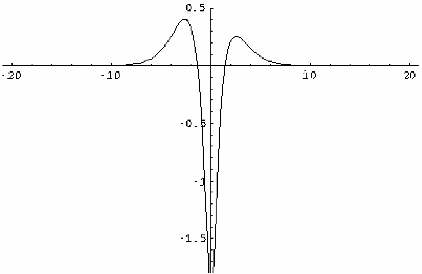
Figure 4b. Motion of a double pole solution at t = 0 with \alpha = 6 and \delta = 1
