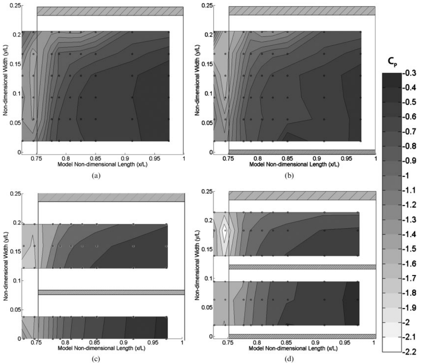
Fig. 13 Contours of the pressure for (a) the plane, (b) the two-channel, (c) the three-channel, and (d) the four-channel 16° diffusers at 28 mm ( x/L = 0.0903 )
