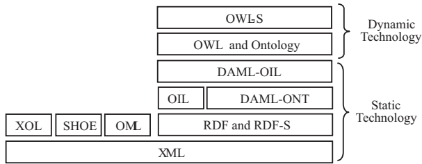
Fig. 3 Different ontology languages proposed in literature
