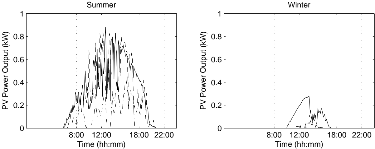
Figure 5: Examples of the simulated PV power generation of a 10m 2 PV system against time of day for 3 days in summer left, and 3 days in winter, right. The 1 st , 15 th , and 30 th day of each month are plotted.
