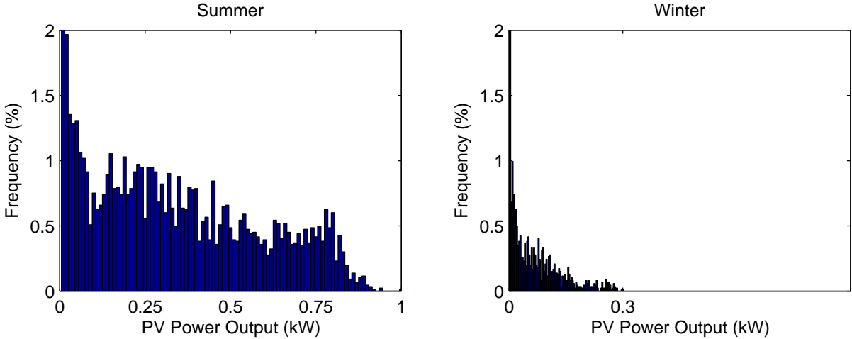
Figure 6: Frequency histograms of the simulated PV power generation of a 10m 2 PV system for summer, left and winter, right. Zero PV power output are excluded in these plots.
