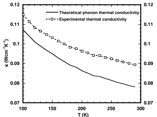
FIG. 6: Deduced \kappa_{ph} and total \kappa of Minami et al thermal conductivity data on YBa_2Cu_3O_{6.93} in the normal state.
