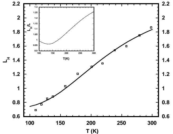
FIG. 3: L_H which fits nicely to experiment ( YBa_2Cu_3O_{6.95} ) using \Theta_b/\Theta_p = 0.36 . This experiment showed a clear violation of the W-F law. The inset gives the ratio of Hall Lorenz number to Lorenz number
