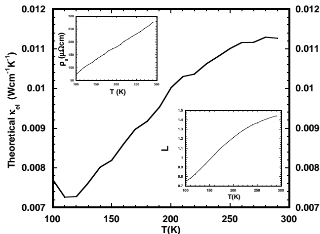
FIG. 5: Normal state \kappa_{el}(= LT/\rho) in optimally doped cuprates calculated using the theoretical L (lower inset) and experimental resistivity data (upper inset).
