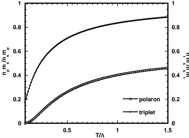
FIG. 2: number density ratios for triplets and polarons in the optimally doped regime
