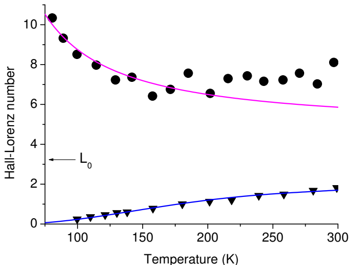
FIG. 1: The Hall-Lorenz number L_H in underdoped twinned EuBa_2Cu_3O_{6.65} (circles)[8] compared with the theory, Eq.(7) when \alpha \ll 1 (upper line), and the significantly different Hall-Lorenz number in detwinned YBa_2Cu_3O_{6.95} (triangles)[5] described by the same theory[7] with a moderate value of \alpha = 0.44 (lower line).
