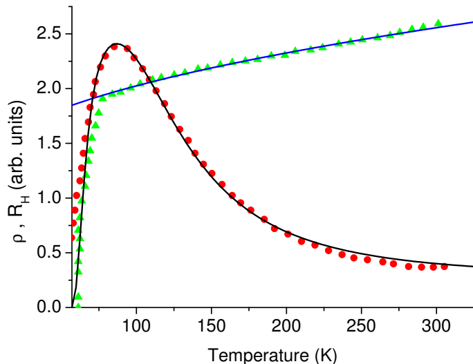
FIG. 2: The in-plane resistivity \rho (triangles) and the Hall ratio R_H (circles) of underdoped twinned EuBa_2Cu_3O_{6.65} , Ref.[8], compared with the theory (lines).
