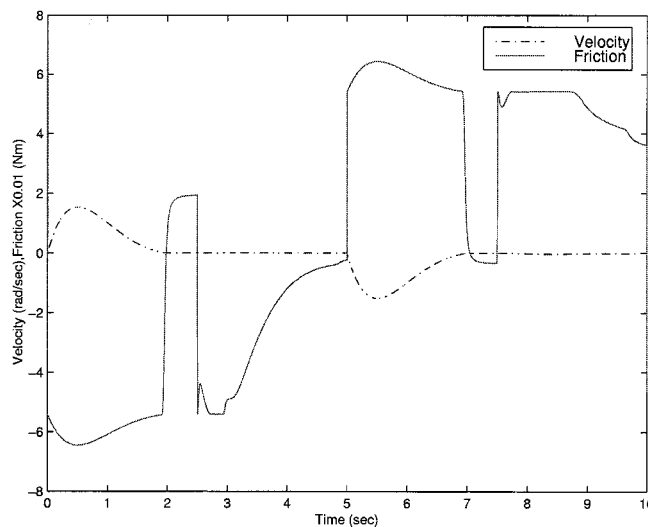
Fig. 3. First-link velocity and friction time histories.
