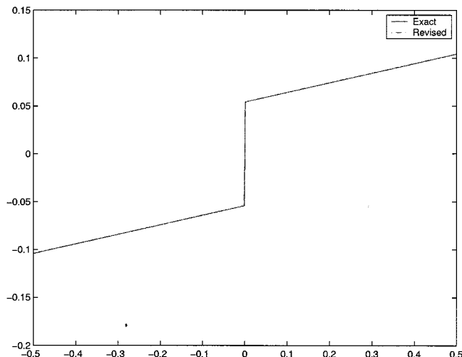
Fig. 2. Comparison of the Columb and Viscous friction model and the revised friction model.
