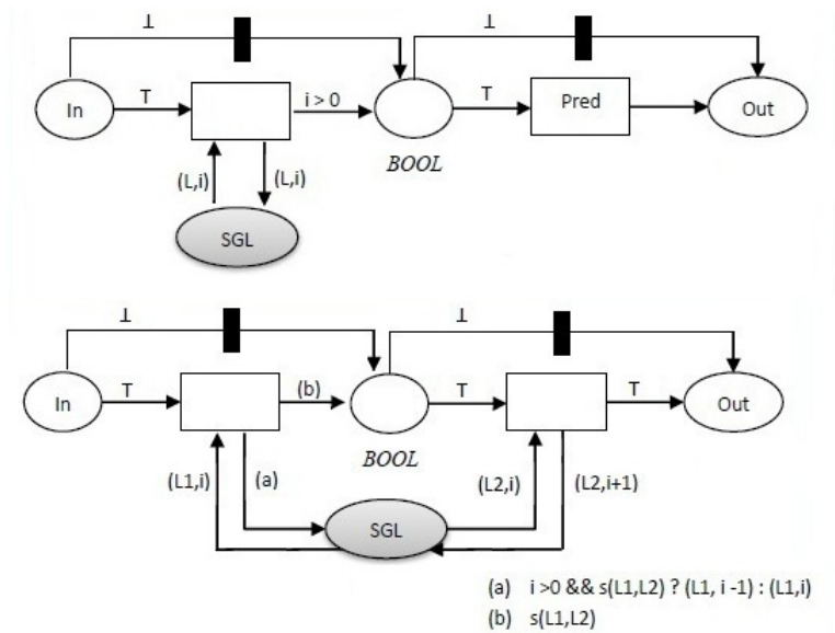
Figure 19: Alternative CPNs for predicate call (up) and move(a, L1, L2) (down).
