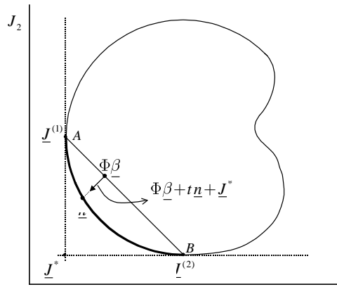
Figure 1. Geometric illustration of NBI Method in 2-dimensional objective space
