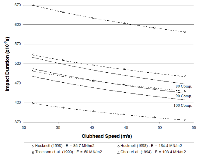
Figure 10. Comparison of experimentally and theoretically obtained values of impact duration calculated from Hertz Law using values of Young's Modulus obtained from four different studies.
