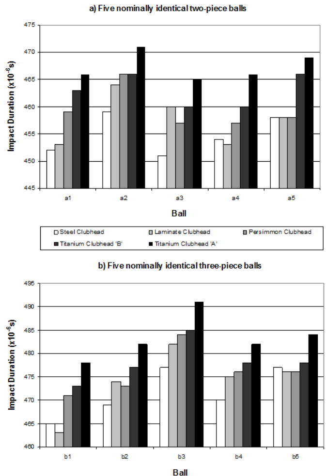
Figure 7. Effects of ball variability and clubhead type on mean impact duration using two sets of balls (a) five nominally identical two-piece balls (b) five nominally identical three-piece balls (Columns are in the same order for each ball, from steel clubhead on the left to titanium clubhead 'A' on the right).
