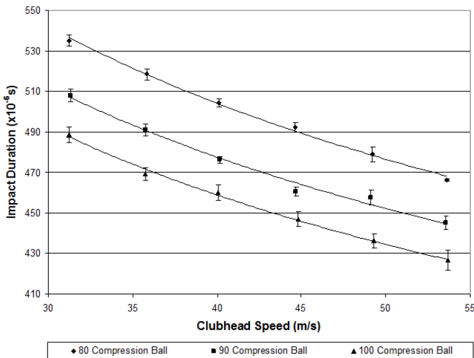
Figure 9. Mean impact durations \pm one standard deviation for three different compression balls hit over a range of clubhead speeds.
