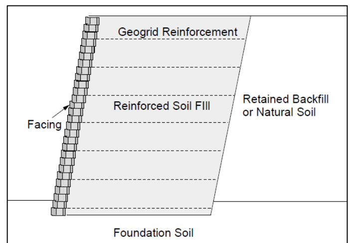
Figure 1. Typical Components in a GRSRS
