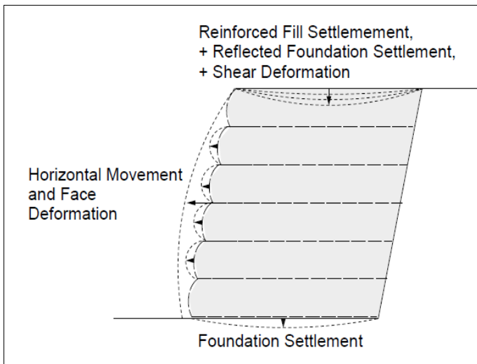
Figure 2. Sources of post-construction deformation in a typical GRSRS according to EBGEO (2011).
