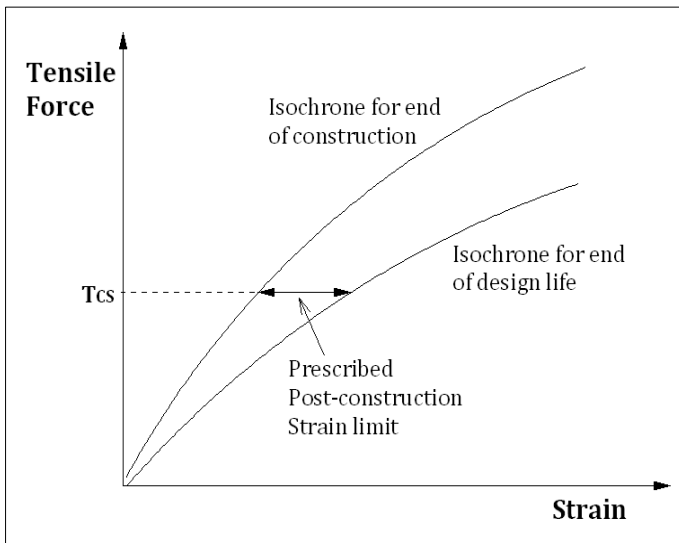
Figure 4. Typical isochronous curve used for restricted service tensile stress capacity. Adapted from BS 8006 (2010).
