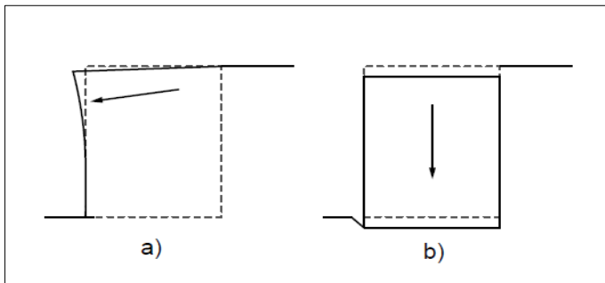
Figure 3. Serviceability Limit States according to BS 8006 (2010): a) Wall Deformation; b) Settlement.
