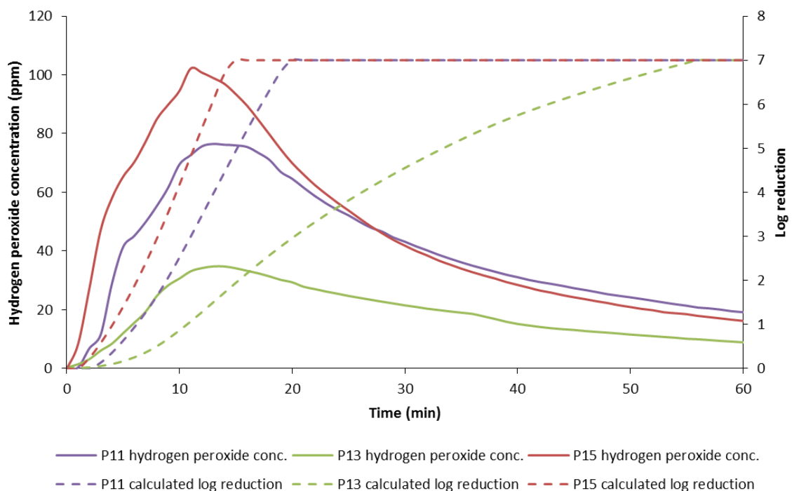
Figure 6.5 High, Mid and Low peak concentration cycles of the hydrogen peroxide decontamination cycle plotted alongside the calculated C. difficile log reduction. Hydrogen peroxide room trace data generated by Keith Schou (Hygienics Biosecurity).
