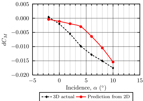
Fig. 33 Prediction of dC_M for a 20% hole with -60 ^\circ obliquity from two dimensional data, with comparison against three dimensional experimental data
