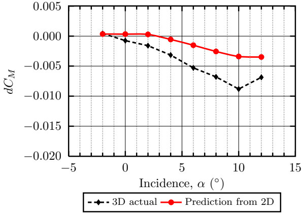
Fig. 31 Prediction of dC_M for a 20% straight through hole from two dimensional data, compared with three dimensional experimental data
