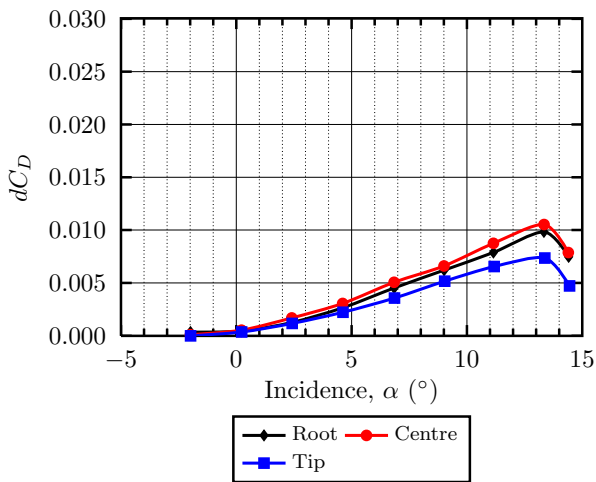
Fig. 8 Variation of dC_D with spanwise location for a 20%c straight through hole
