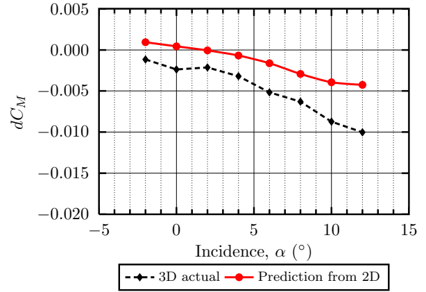
Fig. 34 Prediction of dC_M for a 20% hole with +45 ^\circ skew from two dimensional data, with comparison against three dimensional experimental data
