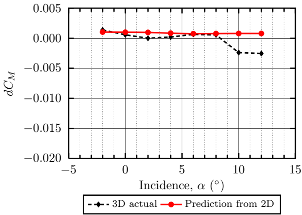
Fig. 32 Prediction of dC_M for a 20% hole with +60 ^\circ obliquity from two dimensional data, with comparison against three dimensional experimental data
