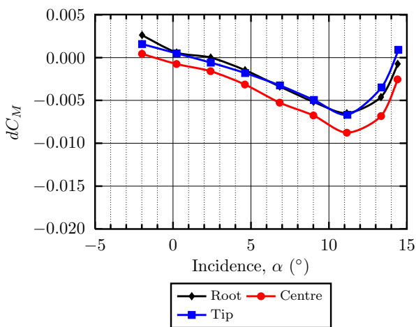
Fig. 9 Variation of dC_M with spanwise location for a 20%c straight through hole
