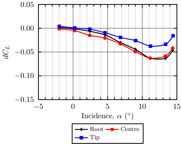
Fig. 7 Variation of dC_L with spanwise location for a 20%c straight through hole
