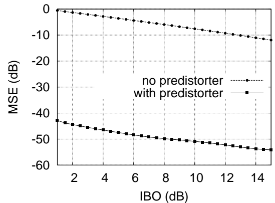
Fig. 10. The mean square error versus IBO performance.
