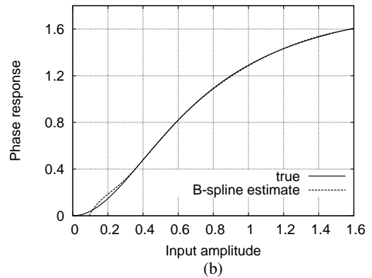
Fig. 7. Comparison of (a) the amplitude response and (b) the phase response between the HPA and the estimated B-spline model, where the HPA operates at the IBO of 0.5 dB with the measurement noise variance 2\sigma_{\xi}^2 = 0.02 .
