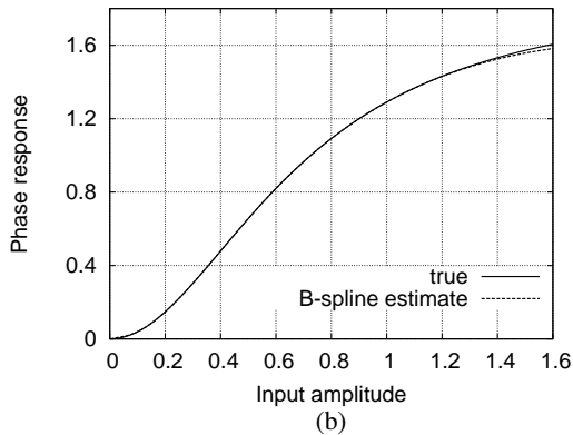
Fig. 6. Comparison of (a) the amplitude response and (b) the phase response between the HPA and the estimated B-spline model, where the HPA operates at the IBO of 5 dB with the measurement noise variance 2\sigma_{\xi}^2 = 0.0 .
