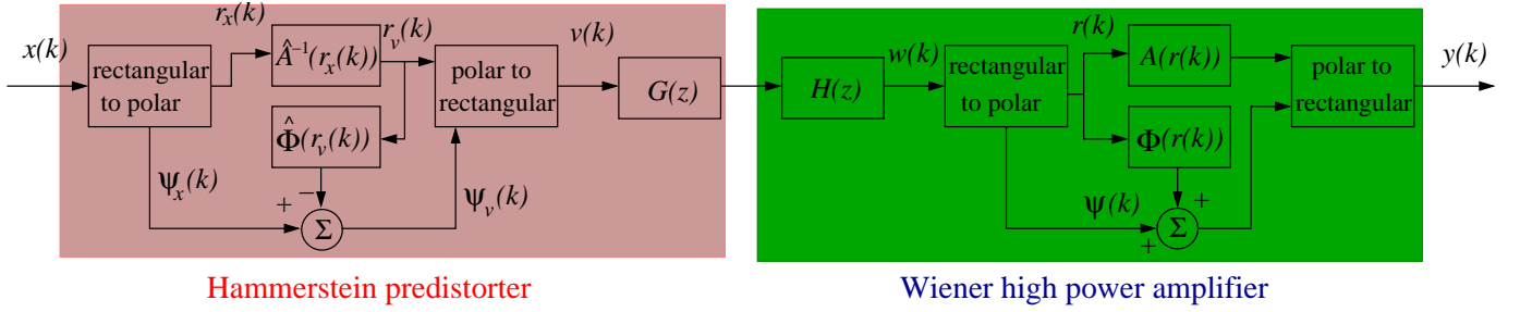
Fig. 2. The predistorter design using the Hammerstein model.
