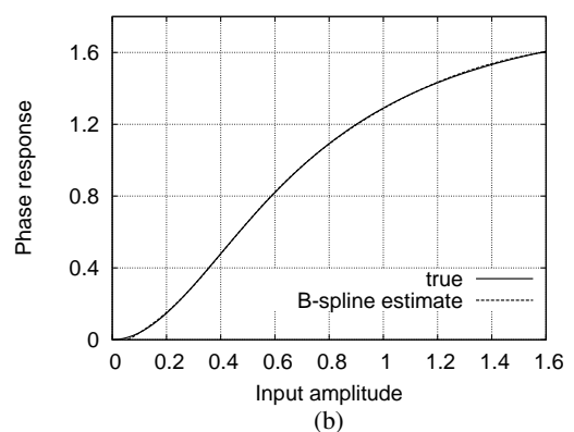
Fig. 8. Comparison of (a) the amplitude response and (b) the phase response between the HPA and the estimated B-spline model, where the HPA operates at the IBO of 0.5 dB with the measurement noise variance 2\sigma_{\xi}^2 = 0.0 .
