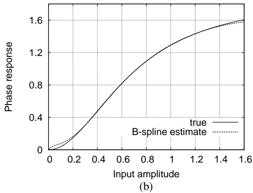
Fig. 5. Comparison of (a) the amplitude response and (b) the phase response between the HPA and the estimated B-spline model, where the HPA operates at the IBO of 5 dB with the measurement noise variance 2\sigma_{\xi}^2 = 0.02 .
