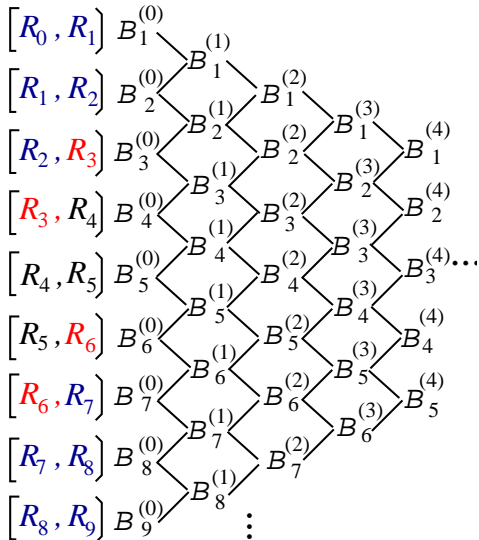
Fig. 1. Visualisation of the De Boor recursion for P_o = 4 and N_b = 5 .
