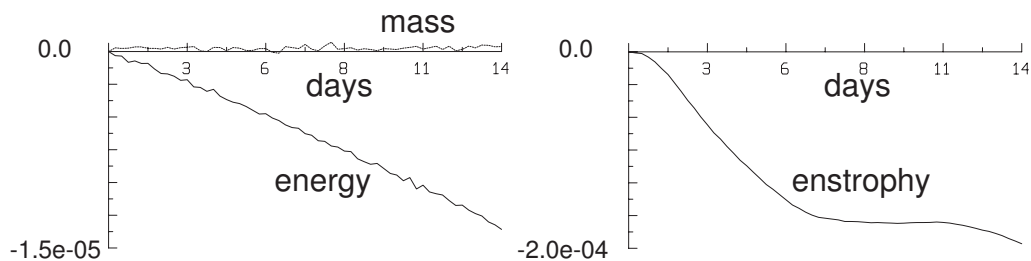
Fig. 13. Mass, energy and potential enstrophy conservation errors, in single precision, a solution of the Rossby-Haurwitz wave benchmark, using an irregular 7722 points triangular mesh
