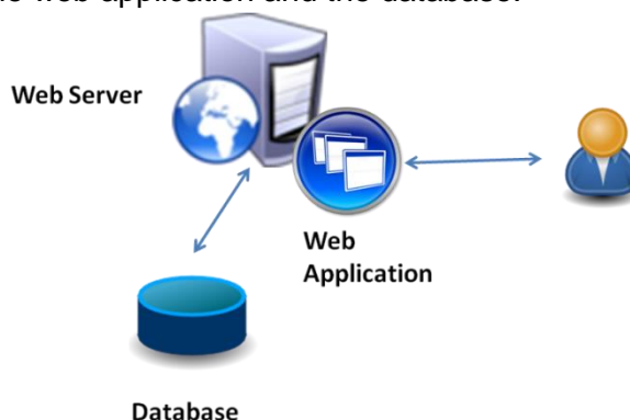
Figure 2.1: Application components
