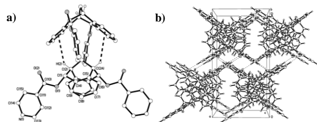
Figure 5 (a) A pair of stacked molecules of ( \pm )- 4c , (b) packing in ( \pm )- 4c showing weak H-bond contacts and overall 3D network. Viewed parallel to the stacking direction.
