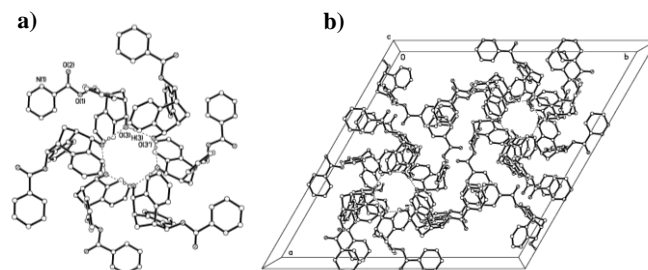
Figure 6 (a) Groups of six molecules of ( \pm )- 4d stacked into a ring and H-bonded, (b) \pi\cdots\pi Stacking of pyridyl groups of neighbouring rings of ( \pm )- 4d molecules.
