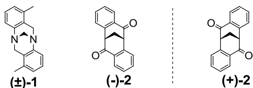
Figure 1. Racemic Tröger's Base (±)- 1 , and (+)- 2 and (-)- 2
