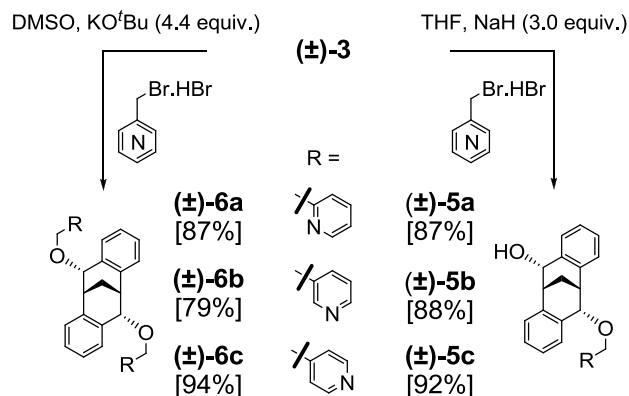
Scheme 3. Selective mono and dietherification of ( ± )- 3 .
