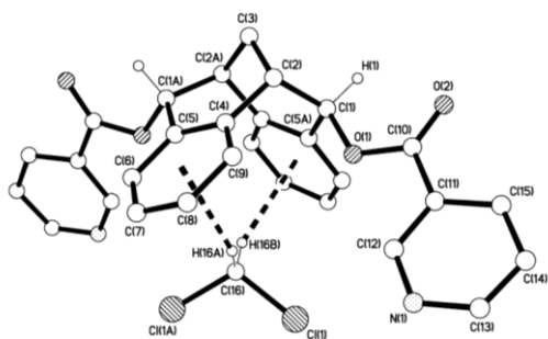
Figure 3. Molecular structure of (+)- 4b ·CH 2 Cl 2 showing pyridyl groups pointing ‘downwards’ into the cleft and the C–H \cdots\pi binding of the dichloromethane solvate.
