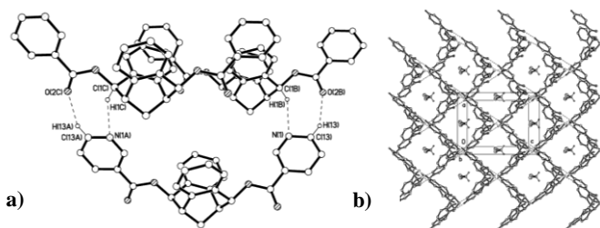
Figure 4 (a) Detail of hydrogen bonding between molecules in (+)- 4b , (b) 3D micro-porous packing with dichloromethane encapsulated within clefts.
