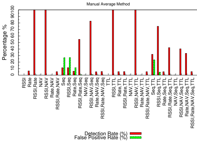
Fig. 3. Results for Rogue AP attack using Manual method and considering data frames
