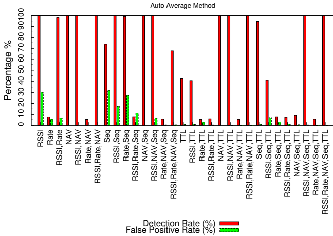
Fig. 4. Results for Rogue AP attack using Automatic method and considering data frames
