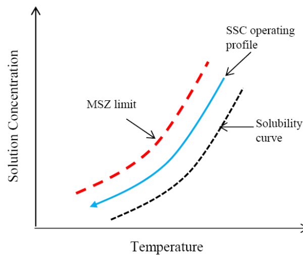
Figure 4.1: Operating curve for supersaturation control of a seeded batch cooling crystalliser.
