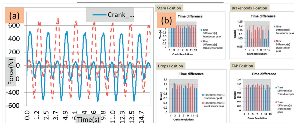
Fig. 3.(a) Radial forces measured at the right and left cranks; (b) Crank revolution indicative times for both measuring sources
