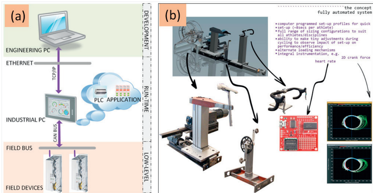
Fig. 1. (a) overview of the system; (b) automated ergometer concept
