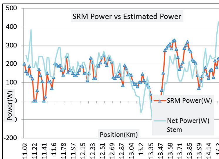
Fig. 2. Comparison of power from road trial versus model
