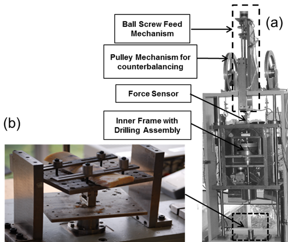
Fig. 4. (a) Drilling Test Rig (b) Mounting of Specimen
