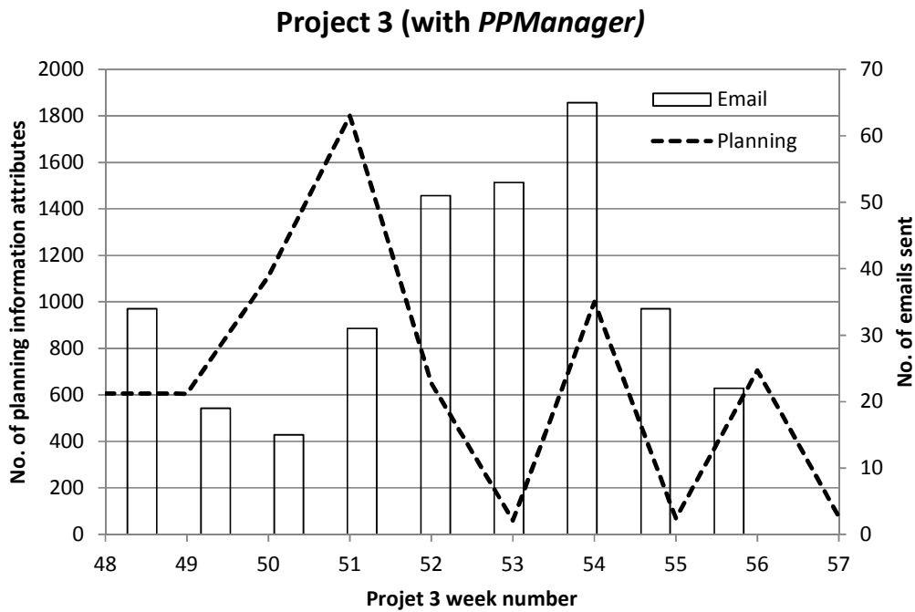
Figure 4 - Planning information attributes transferred during the production phase - Projects 1 and 3
