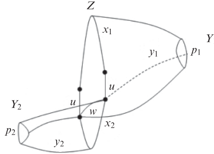
Figure 3. A schematic for the argument that \ker(f) \subset S .
