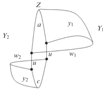
Figure 2. A schematic for the argument that f is surjective.
