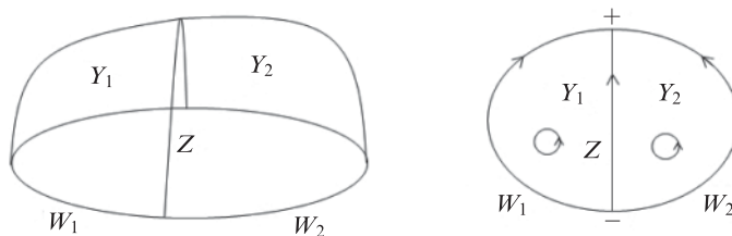
Figure 4. A schematic of a splitting of a \partial -stratified pseudomanifold (left) and a flatter schematic of the relative orientations (right).
