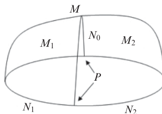
Figure 1. A schematic of the hypothesis of Wall's theorem: The manifold-with-boundary M is split into the pieces M_1 and M_2 along the hypersurface N_0 . The boundary of M is split into N_1 and N_2 along P .
