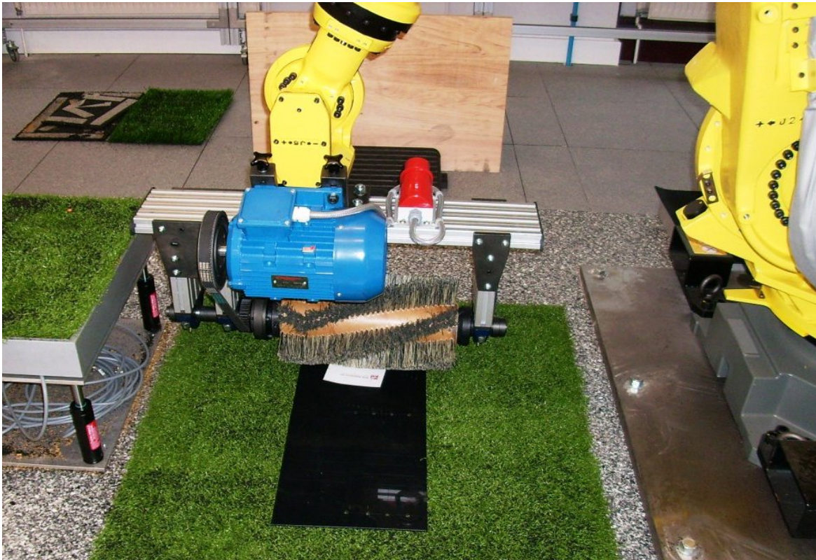
Plate 3 – Fanuc robot arm with power brush mounting (guard removed). The board and paper is to set the penetration depth (see page 9).
