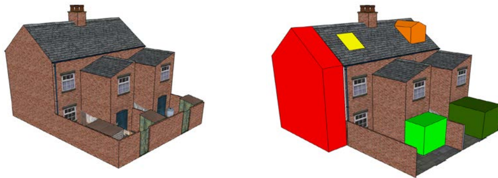
Figure 2: The terrace archetype before and after extension; the colours are assigned to extension types in Table 1.
