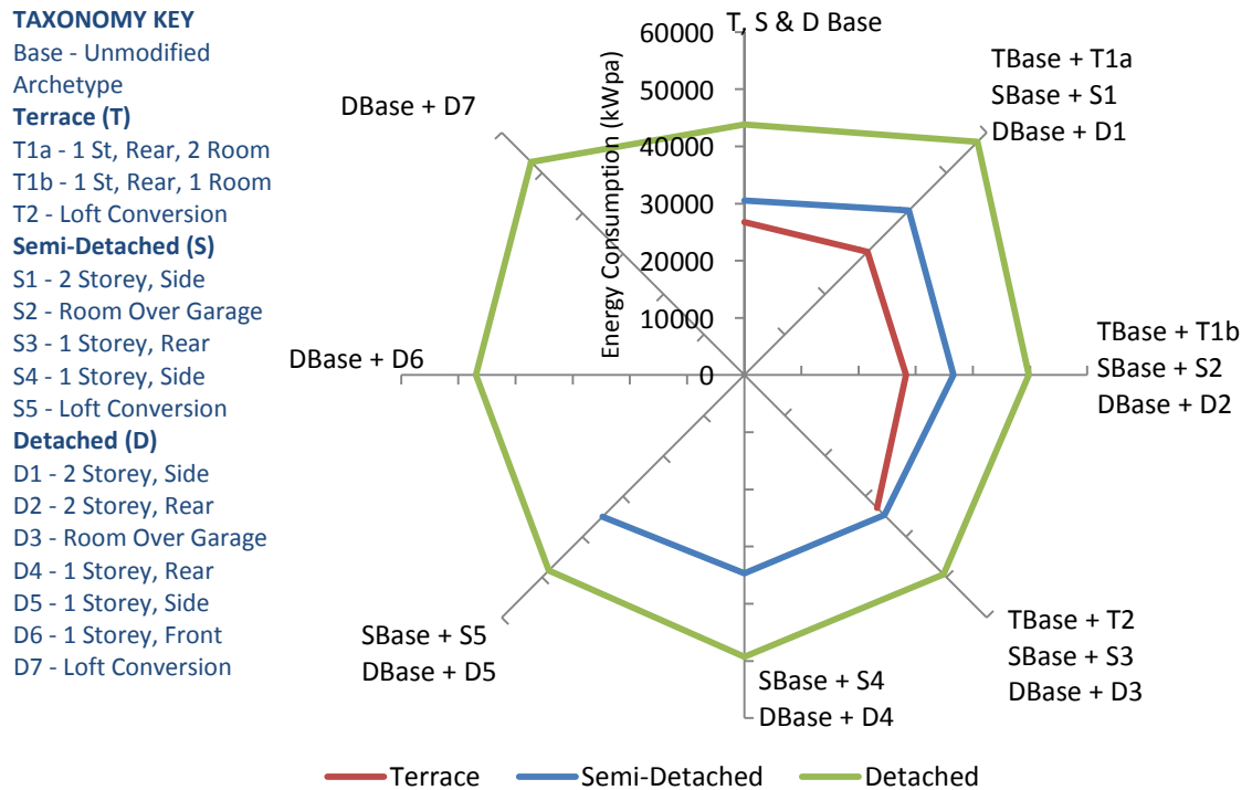
Figure 3: Total energy consumption of each base case and extension combination.
