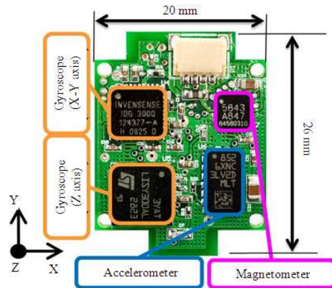
Fig. 1: Inertial measurement unit WB-3
