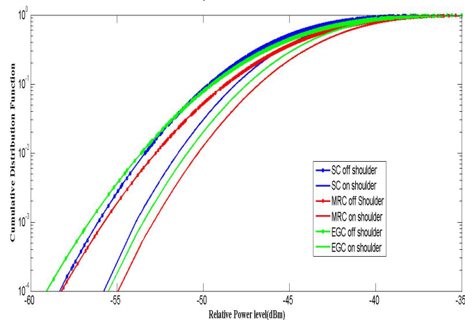
Fig. 6. Selection, Maximal Ratio and Equal gain combining gain results for on and off the shoulder antennas in an office.
