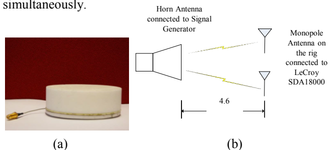
Fig. 2. (a) Quarter wave monopole on a circular groundplane, (b) Schematic of the transmitting and receiving antennas.
