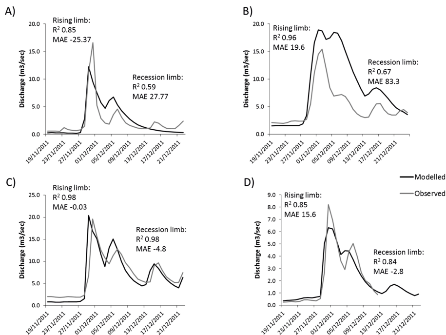
Figure 7. Analysis of INCA model fit to event data at outflow of (a) Holland, (b) Pefferlaw, (c) Beaver and (d) Whites catchments. Rising and recession limb at analysed separately for R^2 and model average error (MAE) to determine model performance under precipitation events. All events were analysed during the same four day period of intense precipitation in November 2011. Although event curves can be used to confirm model representation of reality, it should be noted they should not be used to compare response times between catchments.
