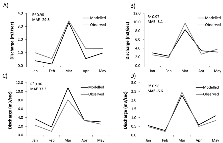
Figure 8. Analysis of model response to observed spring melt in (a) Holland, (b) Pefferlaw, (c) Beaver and (d) Whites catchments. Results analysed during spring melt of 2010.
