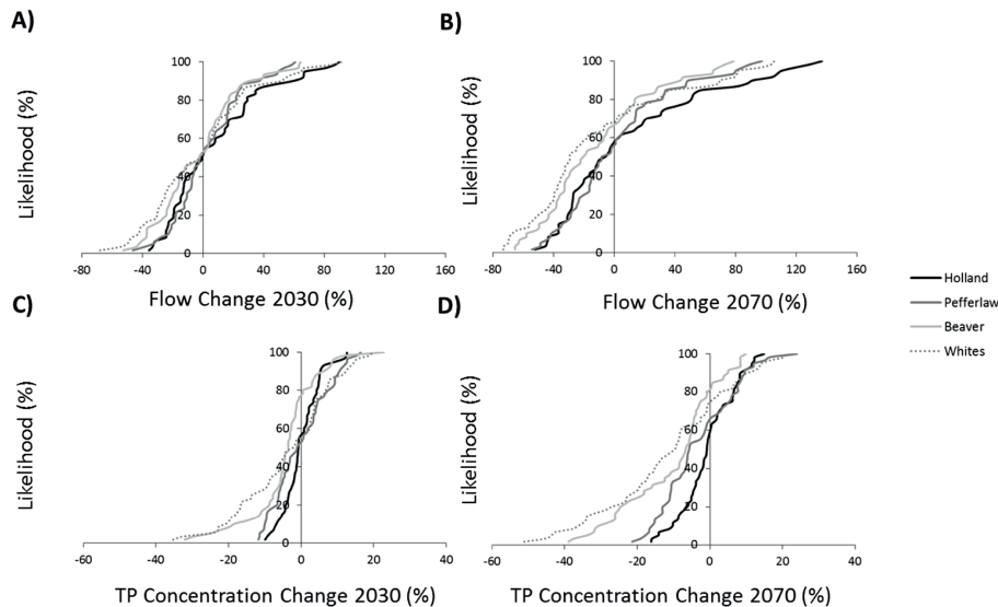
Figure 10. Between-catchment comparison of the CDFs from the perturbed physics ensemble of (a) monthly change in flow by 2030, (b) monthly change in flow by 2070, (c) monthly change in total phosphorus (TP) concentration by 2030, (d) change in TP concentration by 2070 (CDF: cumulative distribution function).
