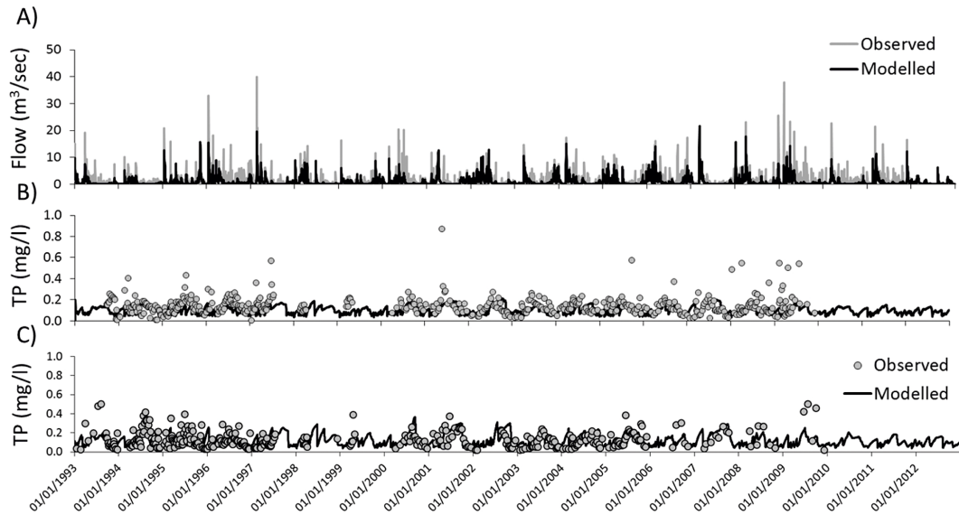
Figure 5. Example of INCA model output. Calibration results from Holland River comparing modelled and observed data of (a) flow at East Branch outflow, (b) total phosphorus (TP) concentrations at East Branch outflow, (c) TP concentration at West Branch outflow.
