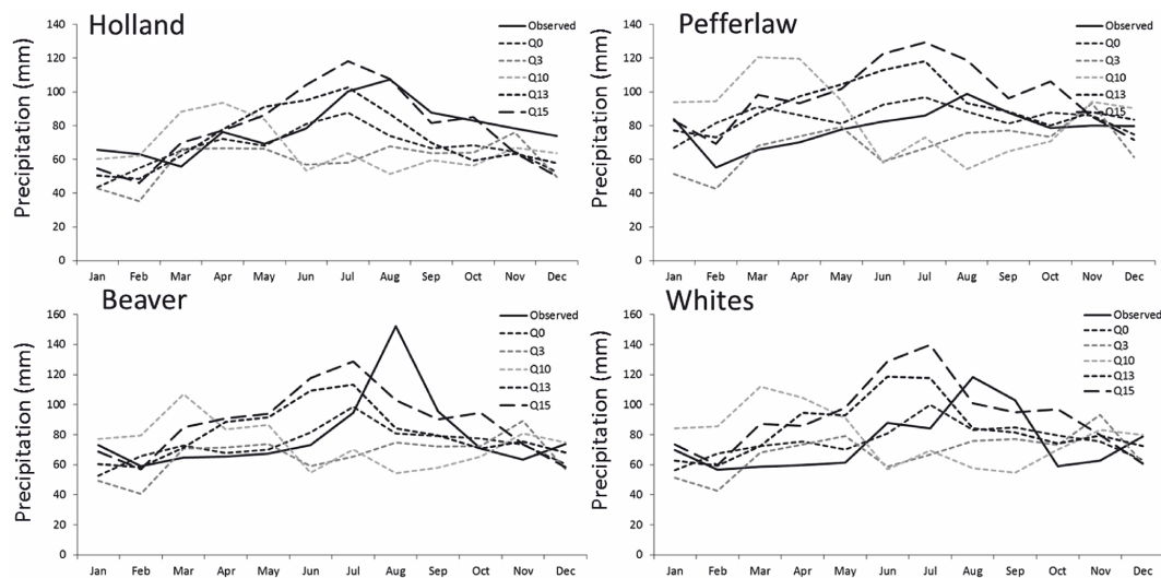
Figure 3. Comparison of monthly precipitation data from 5 ensemble members (Q0–Q15), regionally downscaled using PRECIS, with observed meteorological station data over 30 year baseline period (1968–1997).
