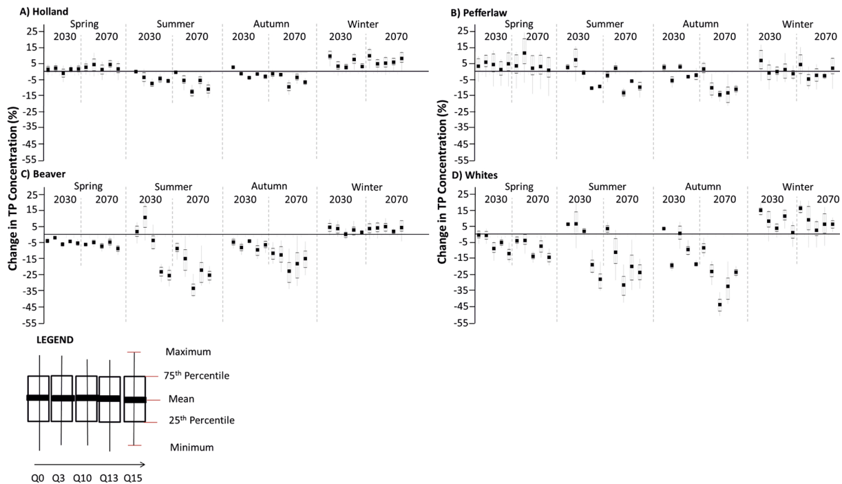
Figure 12. Box plot of seasonal changes in total phosphorus concentrations across all perturbed physics ensemble members (one box per ensemble member) in (a) Holland, (b) Pefferlaw, (c) Beaver and (d) Whites.
