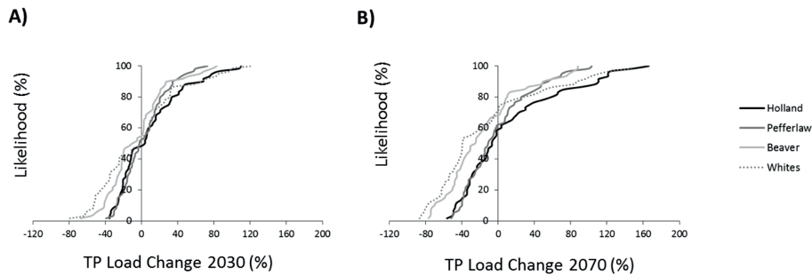
Figure 11. Between-catchment comparison of the CDFs from the perturbed physics ensemble of (a) change in total phosphorus loads (TP) by 2030, (b) change in TP loads by 2070 (CDF: cumulative distribution function).
