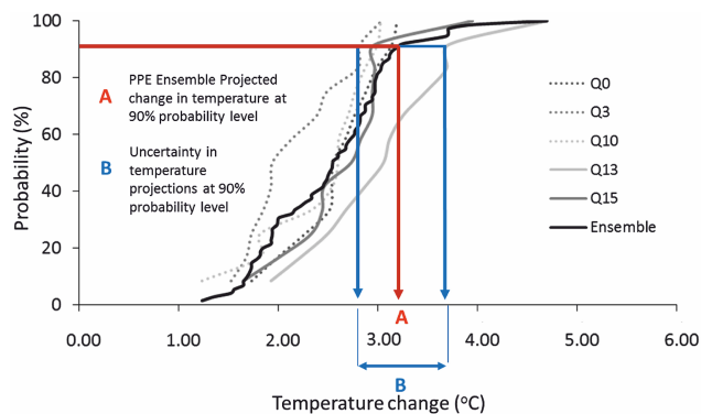
Figure 4. Calculations of (a) monthly change in temperature and (b) projected uncertainty from cumulative distribution functions of perturbed physics ensemble temperature data of the Holland River in 2030.
