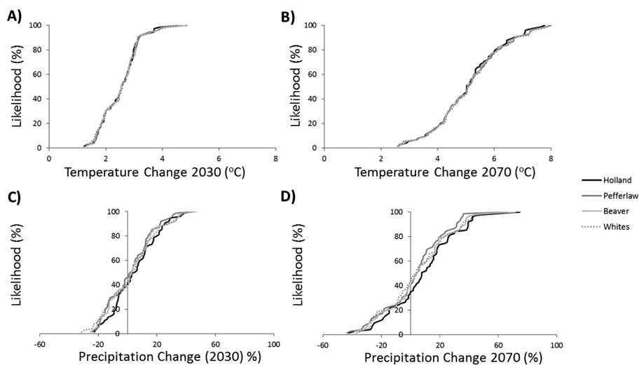
Figure 9. Between-catchment comparison of the CDFs from the perturbed physics ensemble of (a) monthly change in temperature by 2030, (b) monthly change in temperature by 2070, (c) monthly change in precipitation by 2030, (d) monthly change in precipitation by 2070 (CDF: cumulative distribution function).
