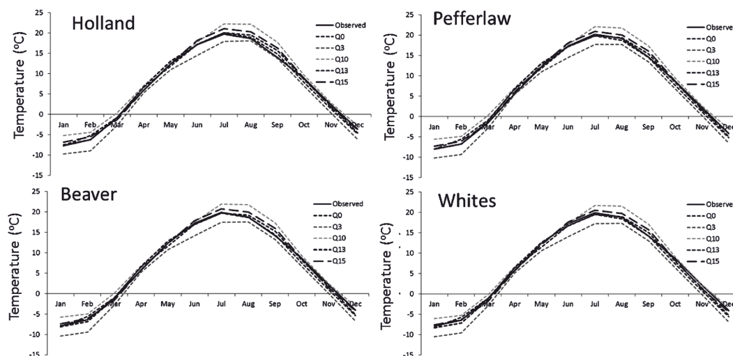
Figure 2. Comparison of monthly temperature data from 5 ensemble members (Q0–Q15), regionally downscaled using PRECIS, with observed meteorological station data over 30 year baseline period (1968–1997).
