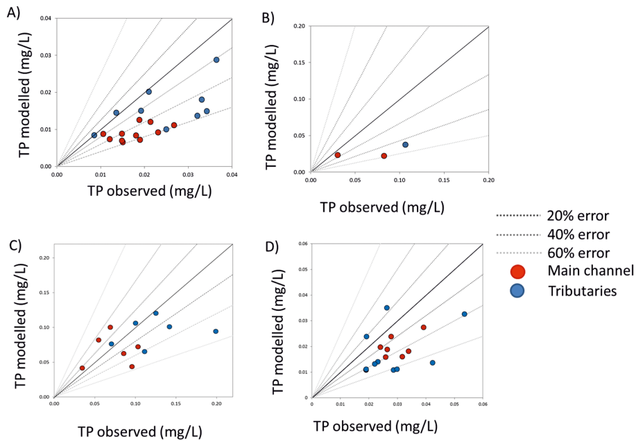
Figure 6. Spatial variability in model accuracy of total phosphorus (TP) concentrations throughout INCA models calibrated across multiple reaches, illustrating relative model error in (a) Holland, (b) Pefferlaw, (c) Beaver and (d) Whites catchments. Data represents average TP concentrations over the calibration period.
