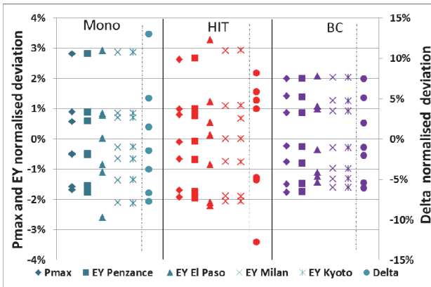
Fig 2. Pmax, EY and Delta deviation for each module.
