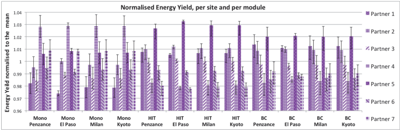
Fig 1. Energy Yield deviation normalized to the mean for each site and module. The error bars represent the best and worst case scenario in energy yield based on the LIC measurement deviations between the partners.
