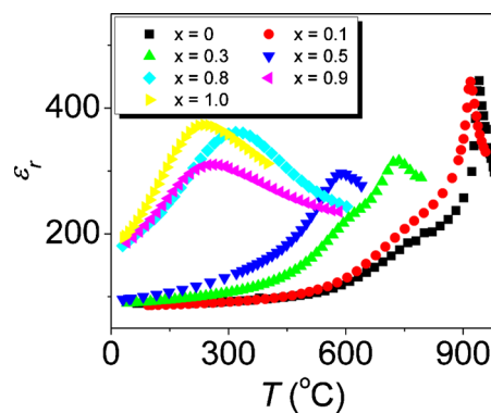
FIG. 4. (Color online) Temperature dependence of dielectric constant of (\text{CBNO})_{1-x}(\text{BBNO})_x ceramics at the frequency of 1 MHz.
