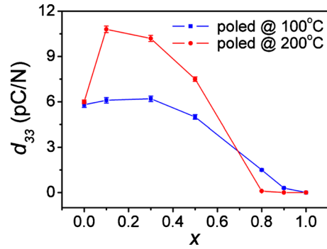
FIG. 8. (Color online) Piezoelectric coefficient ( d_{33} ) as a function of x for (\text{CBNO})_{1-x}(\text{BBNO})_x ceramics poled at different temperatures ( 100^\circ\text{C} and 200^\circ\text{C} ).
