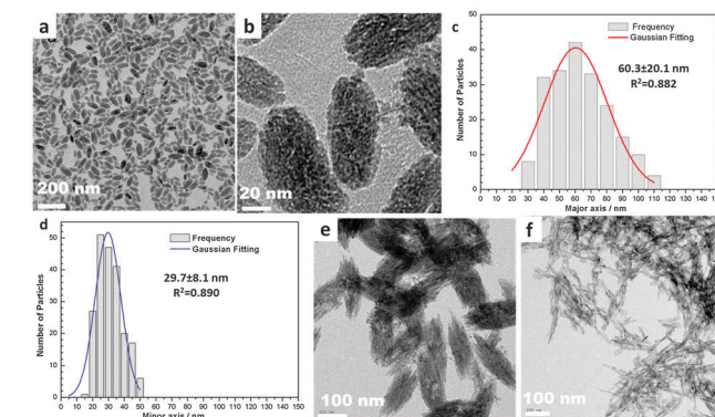
Fig. 1 TEM images (a) and (b) and size distribution (c) and (d) (major and minor axis, respectively) of Fe 3 O 4 @HA NPs synthesised from Fe 3 O 4 @Al(OH) 3 in the presence of BP-PEG-Me; (e) TEM image of MnFe 2 O 4 @HA NPs synthesised in absence of BP-PEG-Me 2 ; (f) TEM image of pure HA NPs.
