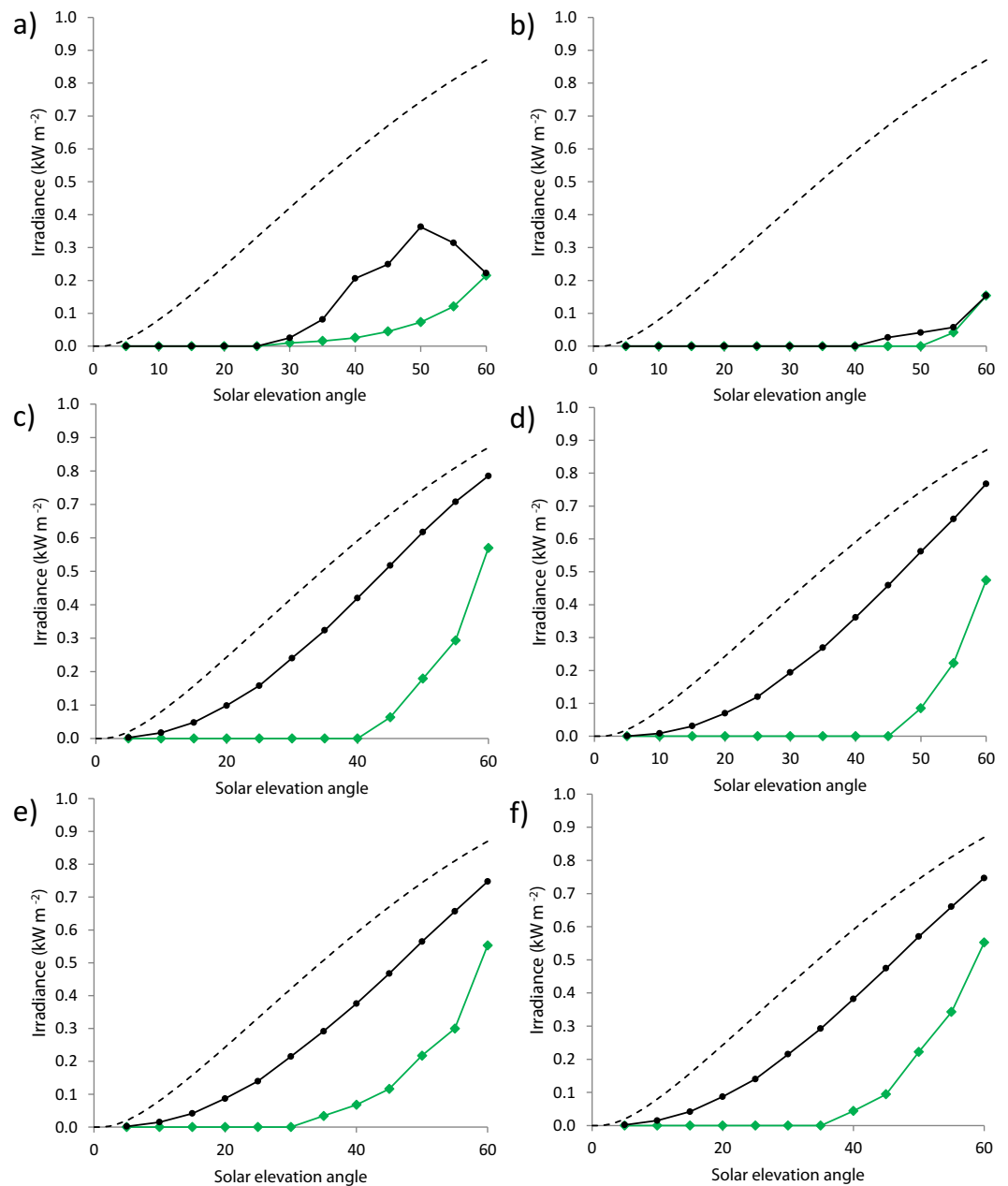
Figure 5. The irradiance ( \text{kW m}^{-2} ) incident at each solar elevation angle at site D2 (a,b), D10 (c,d), and D16 (e,f) on the River Dove for the rising sun (a,c,e) and setting sun (b,d,f). The black line indicates landscape shade and the green line is landscape plus 20 m high tree shade. The maximum possible radiation at each elevation angle is given by the dashed line.
