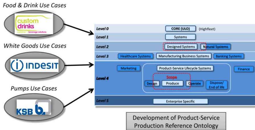
Fig. 6. Use case input into the development of the reference ontology.
