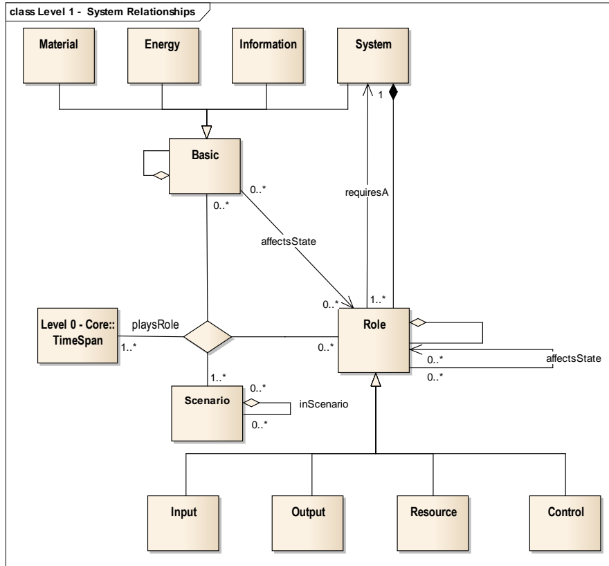
Fig. 4. Global production network reference ontology level 1.
