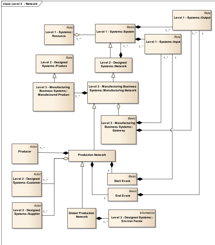
Fig. 5. Level 2 designed systems ontology concepts needed to represent a GPN.
