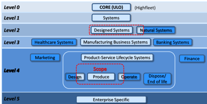
Fig. 3. Global production network reference ontology layers.
