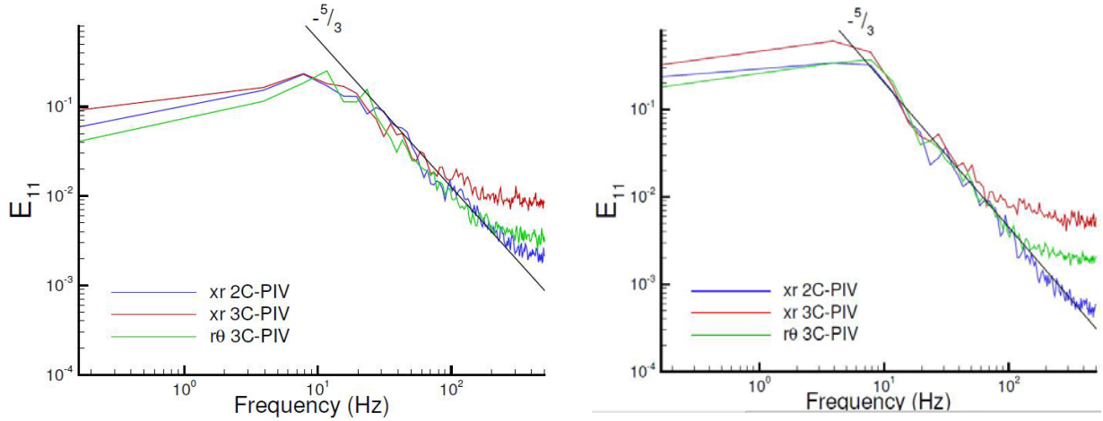
FIGURE 11 (Colour online) PSD of fluctuating axial velocity: r/D_j = 0.5 and x/D_j = 1.5 (left) and 10.0 (right)
