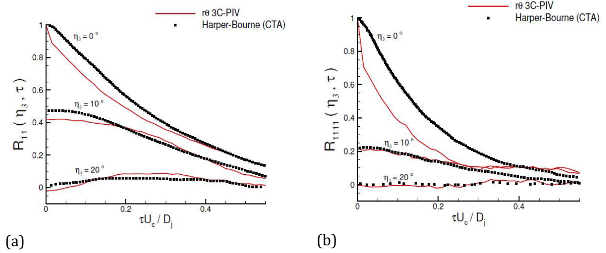
FIGURE 21 (Colour online) R_{11} and R_{11,11} plots for azimuthal separations at D_j = 4.0 , r/D_j = 0.5
