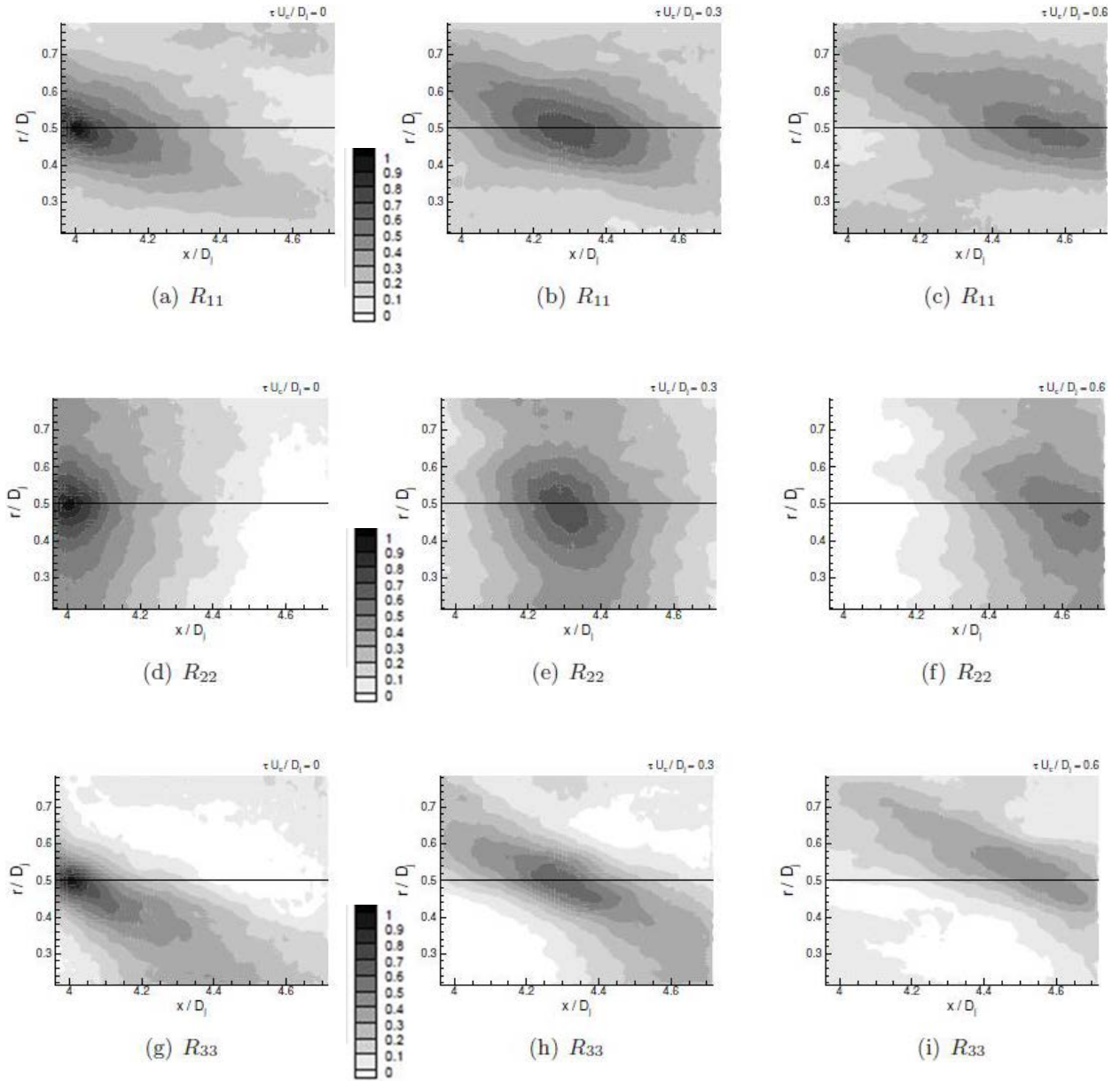
FIGURE 23 2 nd -order spatio-temporal correlations at (4D_j, 0.5D_j, 0^0)
