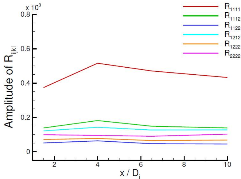
FIGURE 28 (colour online) Axial development of 4 th -order correlation relative amplitudes along shear layer
