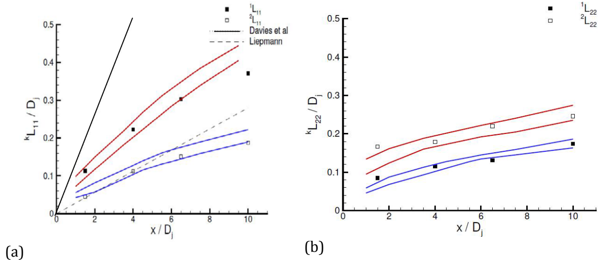
FIGURE 9 (Colour online) Axial (a) and radial (b) lengthscales at r/D_j = 0.5 . Red and blue lines indicate range of data in experiments of Fleury et al. (2008)
