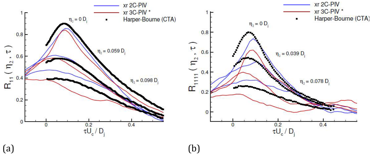
FIGURE 20 (Colour online) R_{11} and R_{11,11} plots for radial separations at D_j = 4.0 , r/D_j = 0.5
