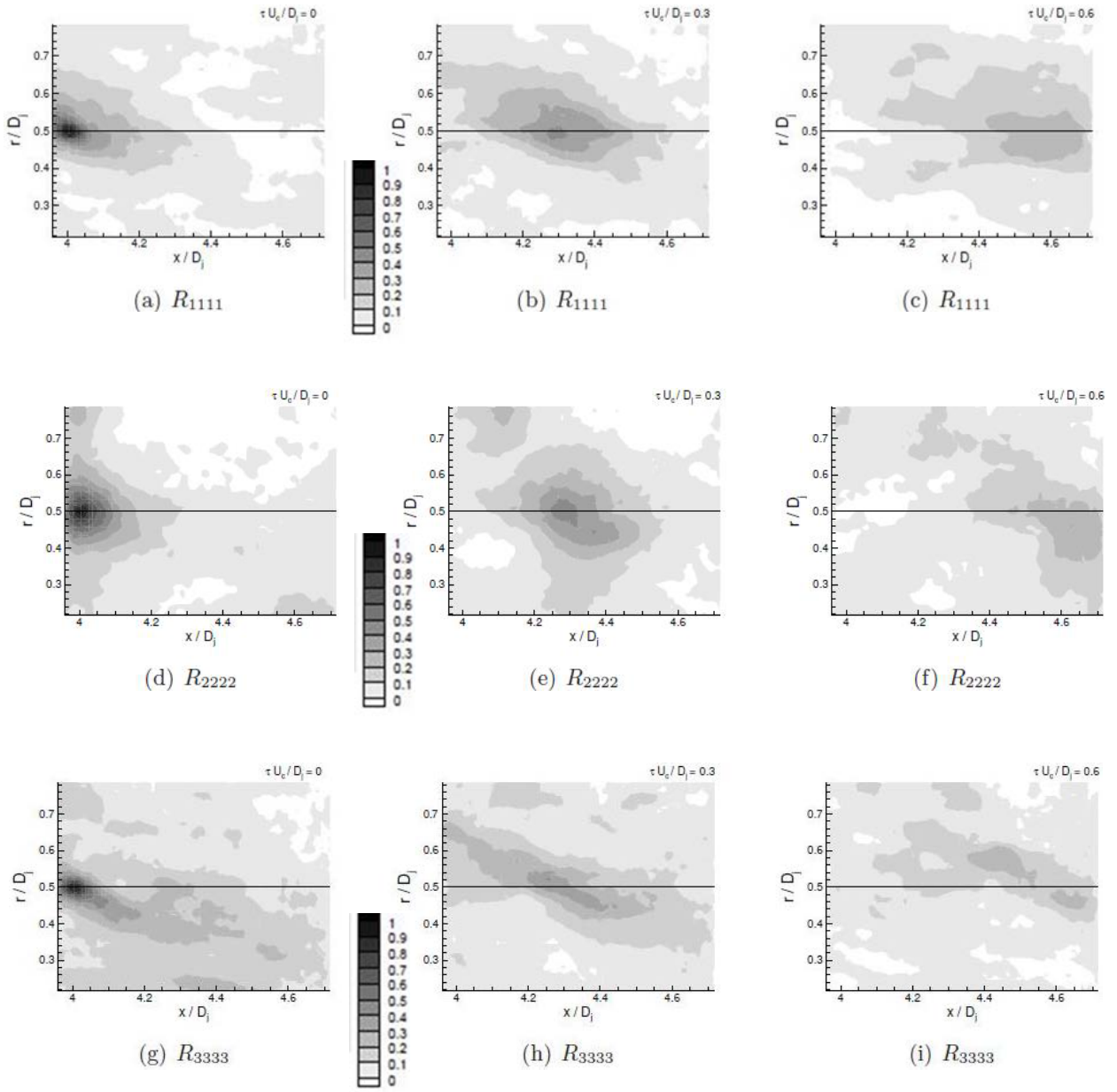
FIGURE 24 4 th -order spatio-temporal correlations at (4D_j, 0.5D_j, 0^0)
