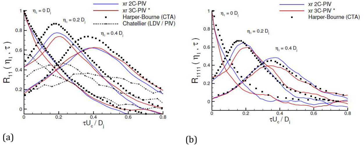
FIGURE 19 (Colour online) R_{11} and R_{11,11} plots for axial separations at D_j = 4.0 , r/D_j = 0.5
