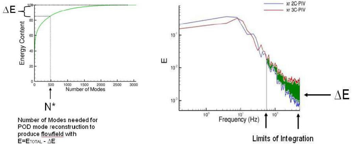
FIGURE 13 (Colour online) Illustration of POD correction method
