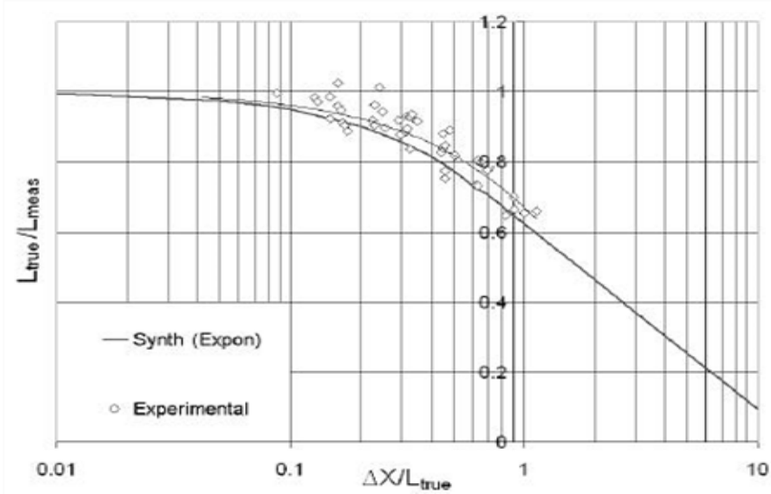
FIGURE 3 Sub-cell filtering correction curves for (a) rms and (b) integral scale (from Spencer and Hollis (2005))
