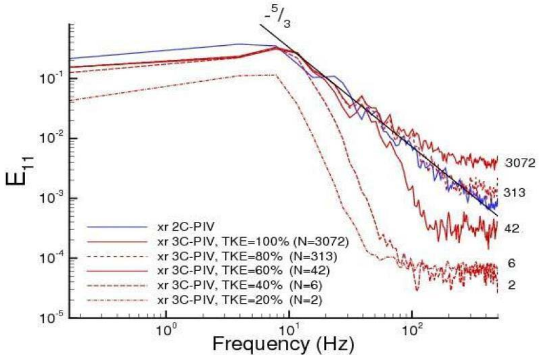
FIGURE 12 (Colour online) Effect of POD mode number on reconstructed PSD (blue – 2C_PIV)
