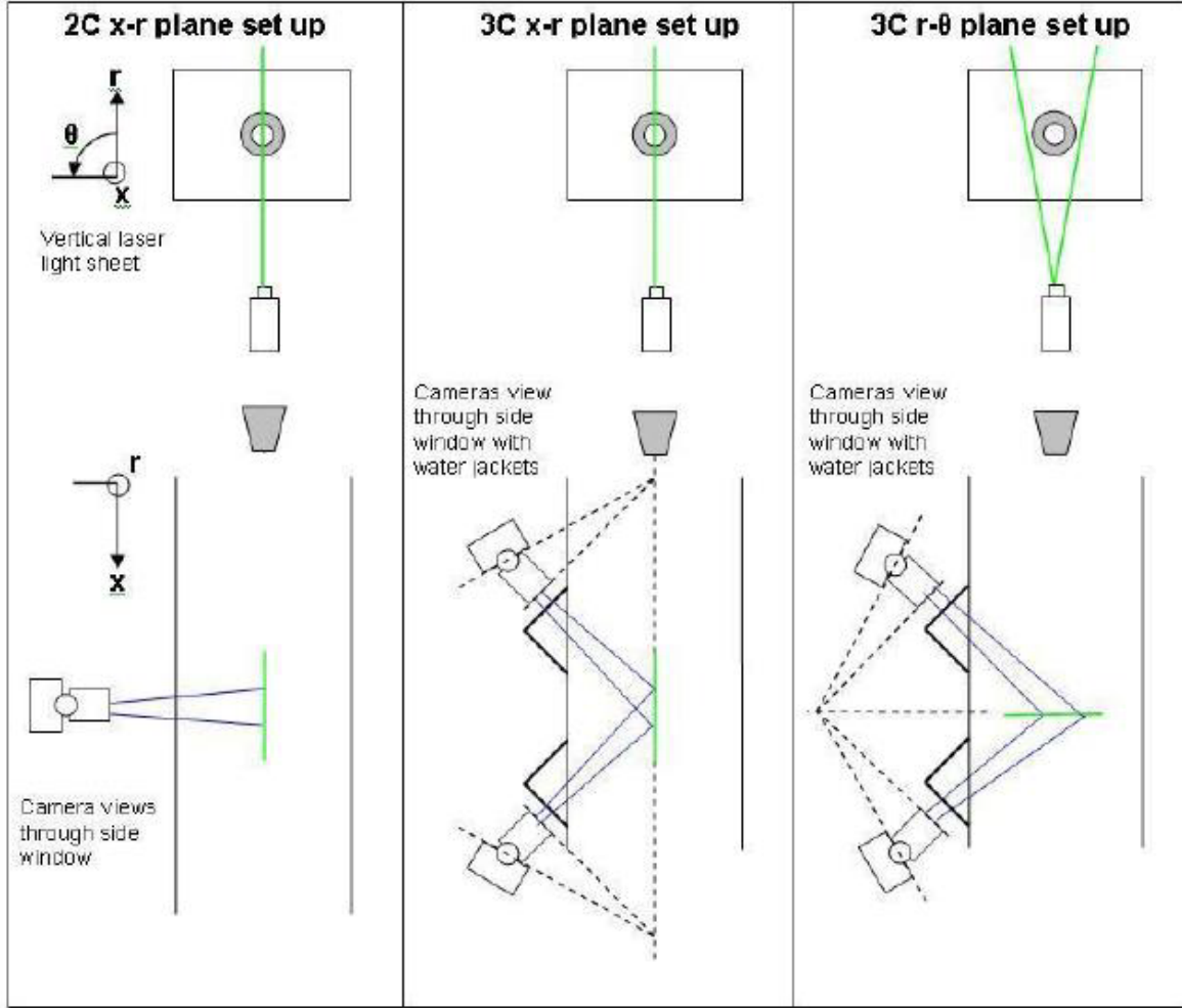
FIGURE 2 (Colour online) Camera and laser locations for various measurement configurations
