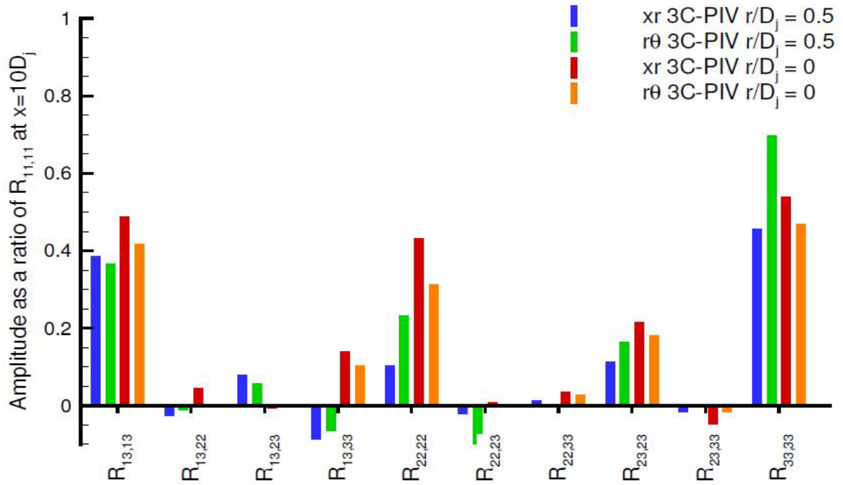
FIGURE 27 (colour online) Comparison of 4 th -order amplitudes relative to R_{11,11} for PIV results
