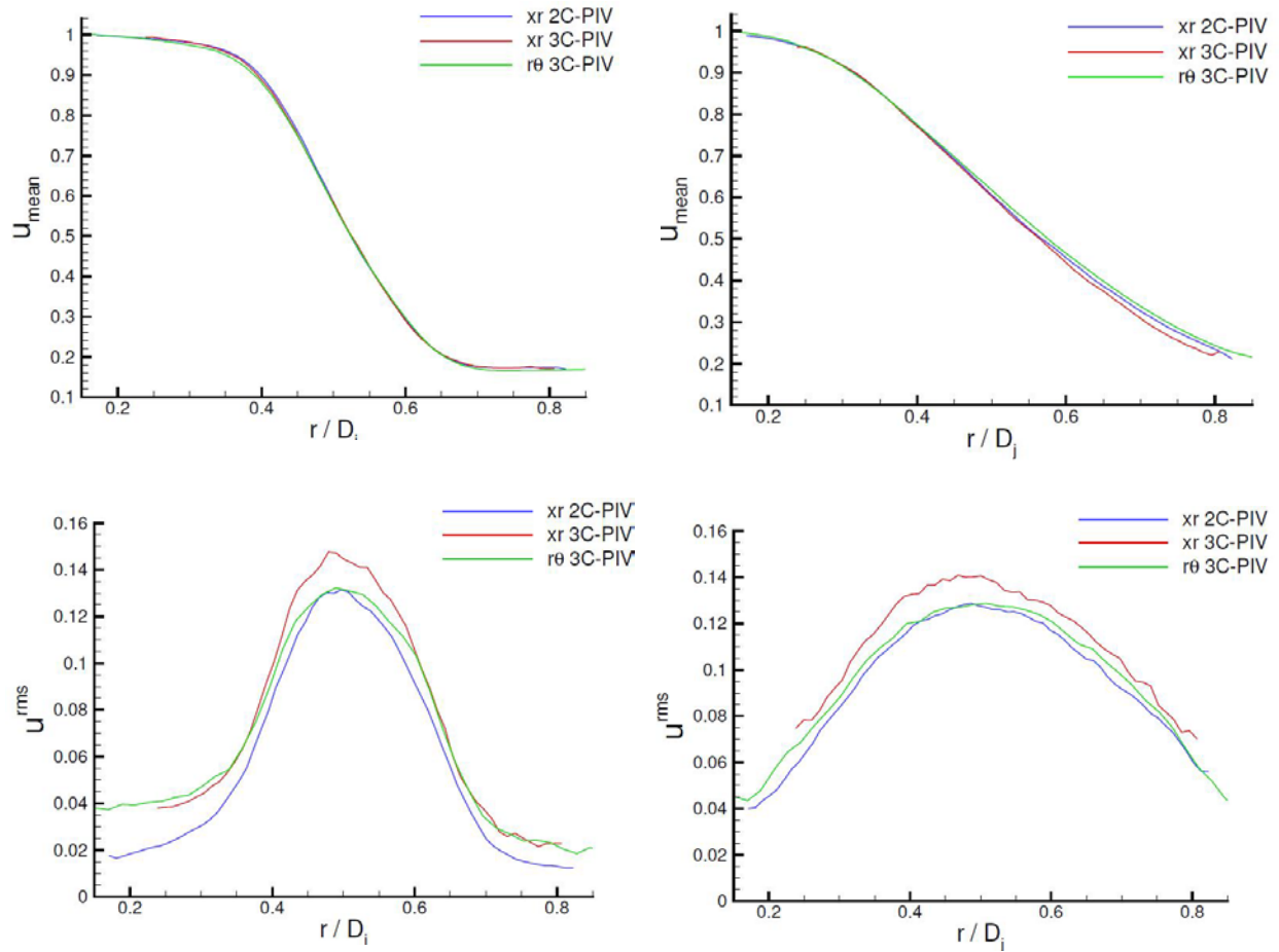
FIGURE 10 (Colour online) Radial profiles: axial mean (top) and rms (bottom) at x/D = 1.5 (left), 4.0 (right) - different PIV configurations
