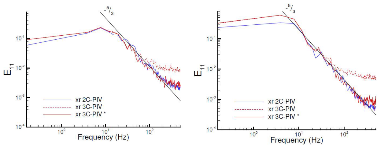
FIGURE 15 (Colour online) Power spectra of axial velocity - comparison of 2C-PIV, 3C-PIV and 3C*-PIV (left) x/D_j = 1.5 , r/D_j = 0.5 , (right) x/D_j = 10.0 , r/D_j = 0.5
