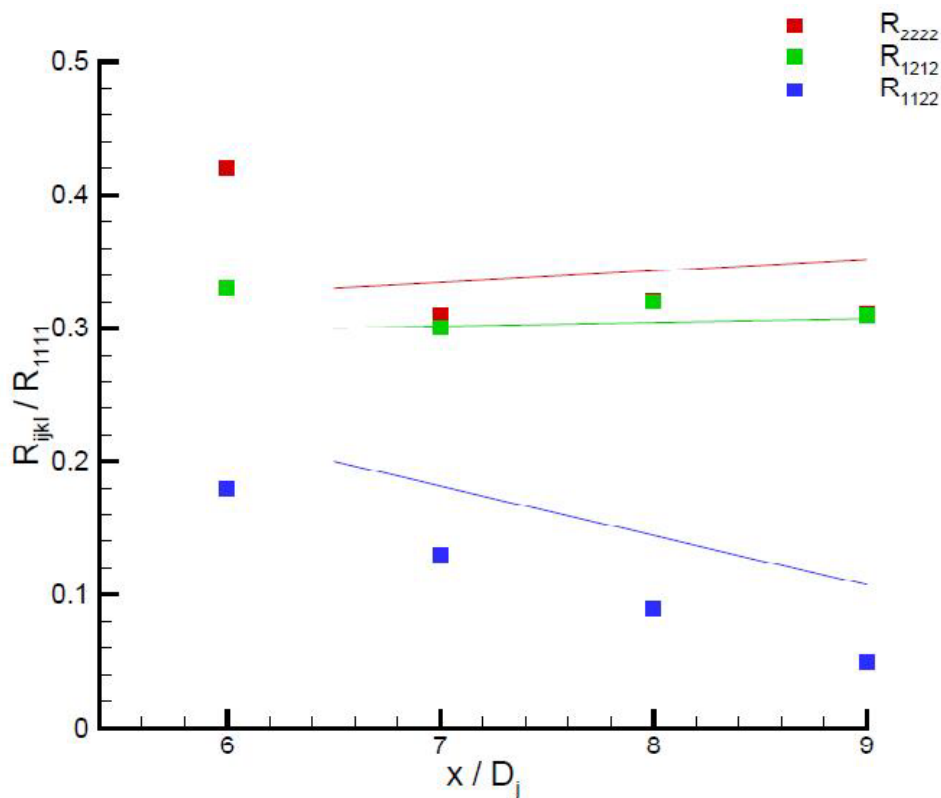
FIGURE 25 (colour online) Comparison of PIV data (symbols) with HWA data Morris & Zaman (2010) (lines) for 4 th -order peak correlation relative amplitudes along jet centreline.
