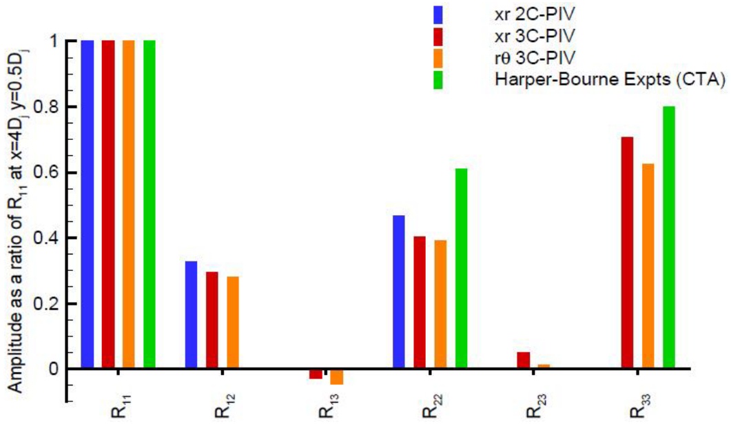
FIGURE 26 (colour online) Comparison of 2 nd -order peak amplitudes relative to R_{11} for PIV and HWA results
