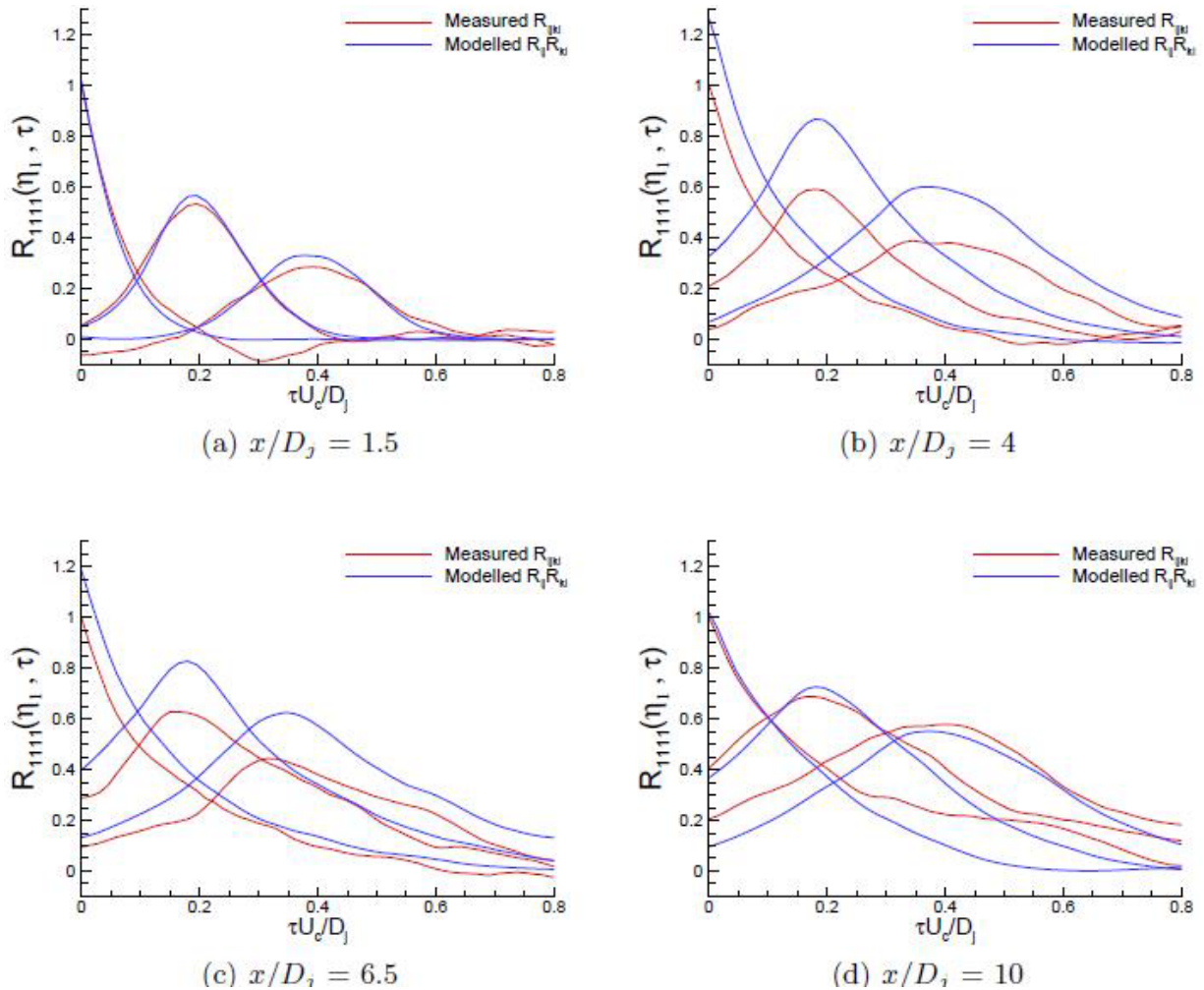
FIGURE 29 (colour online) Comparison between measured and quasi-normal approximation of R_{11,11}
