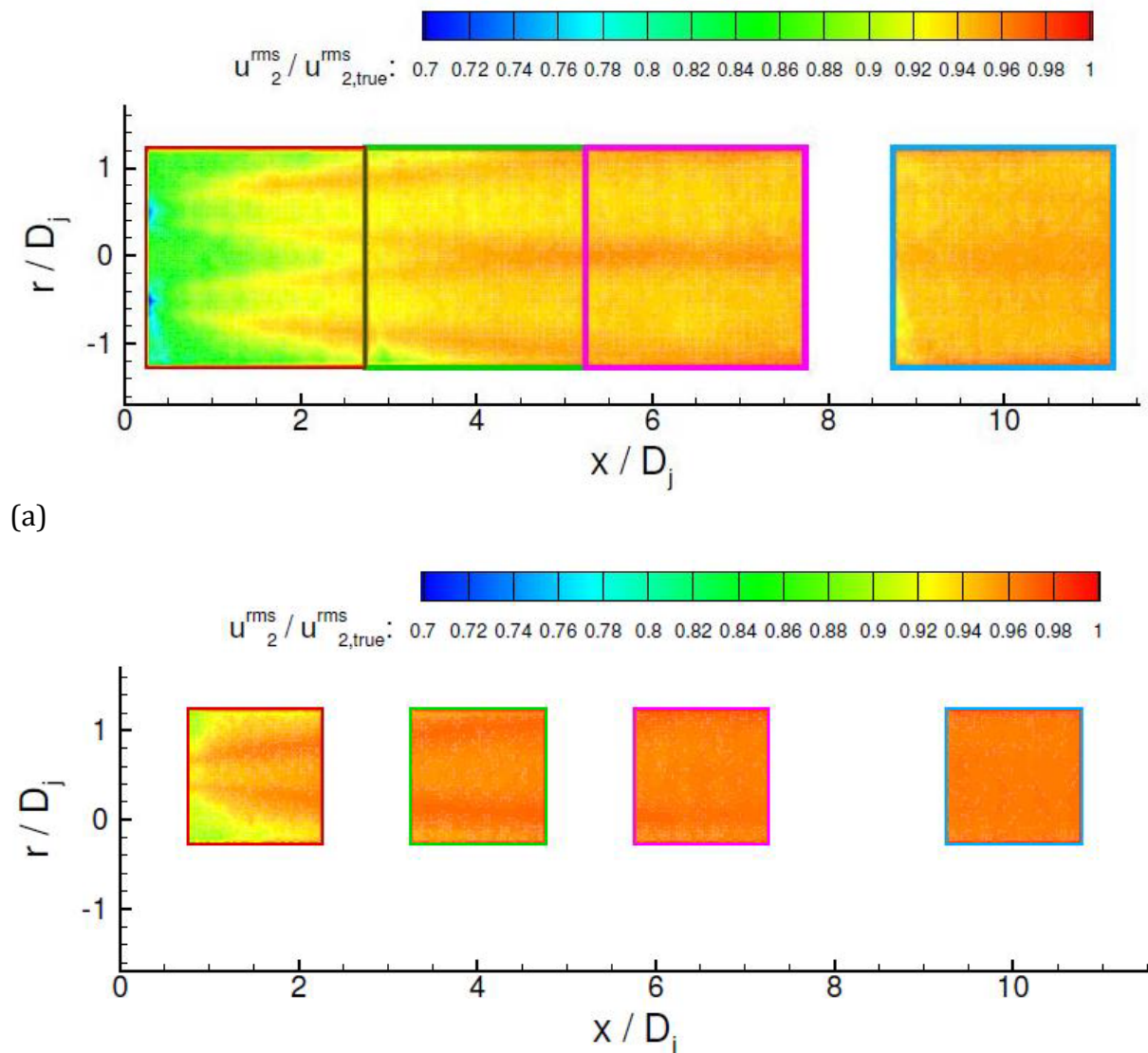
FIGURE 4 (Colour online) Radial rms error maps for FoV sizes: (a) 100x100mm, (b) 60x60mm
