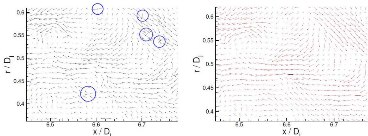
FIGURE 14 (Colour online) Example of instantaneous vector fields at x/D_j = 6.5 , (i) original, (ii) original + POD correction
