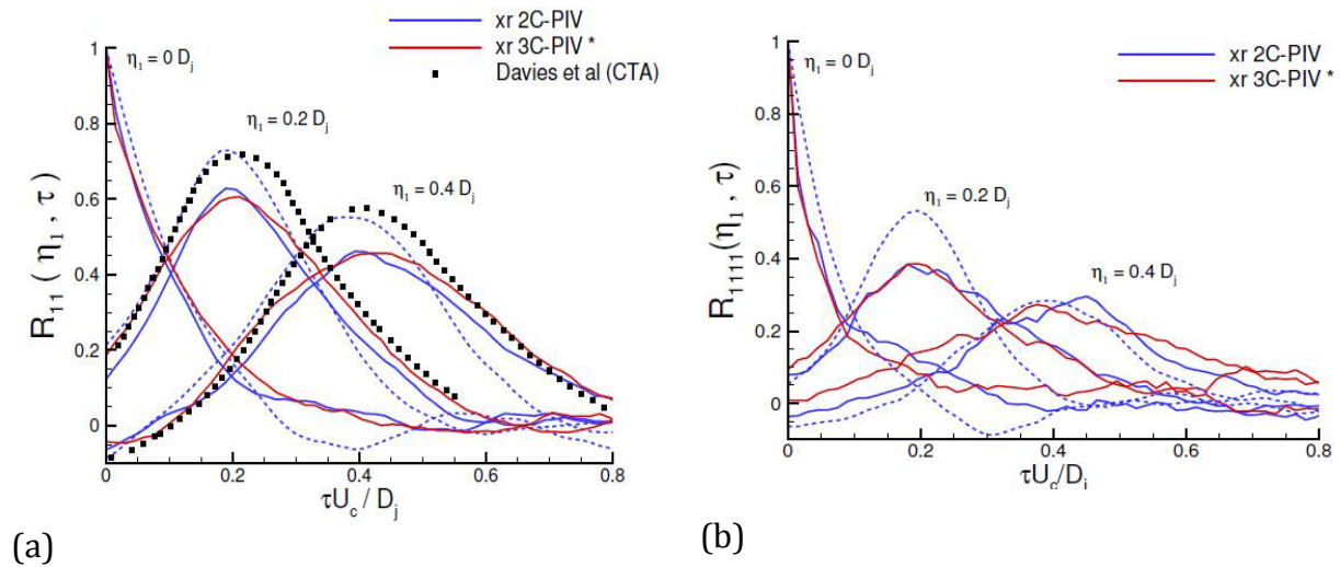
FIGURE 18 (Colour online) R_{11} and R_{11,11} plots for axial separations at x/D_j = 1.5 , r/D_j = 0.5 Solid lines – 25mmx25mm FoV, dashed lines - 40mmx40mm FoV
