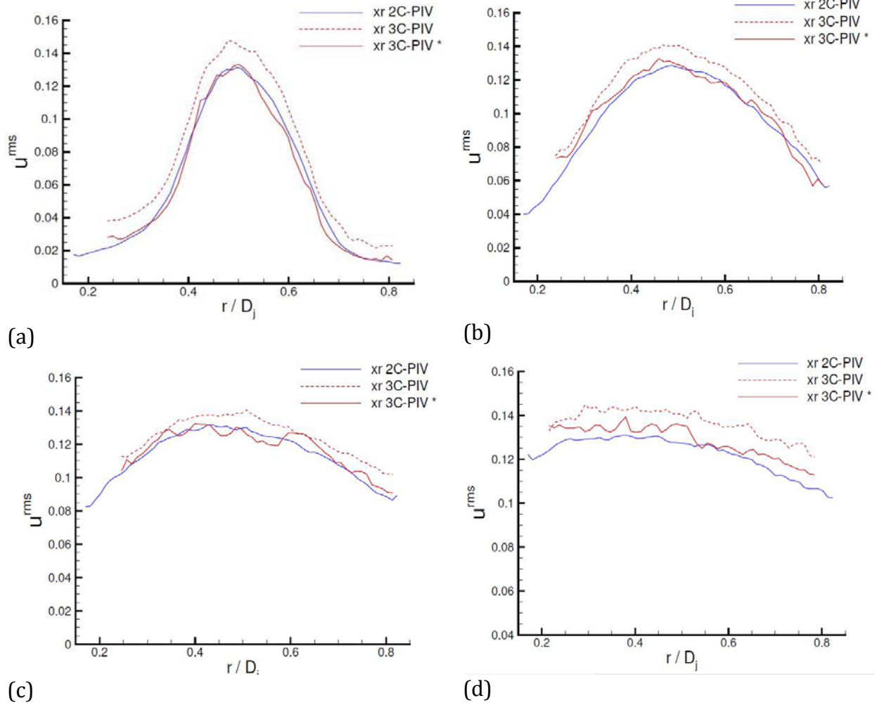
FIGURE 16 (Colour online) Radial profiles of axial RMS fluctuations x/D_j = (a) 1.64, (b) 4.0, (c) 6.5, (d) 10.0
