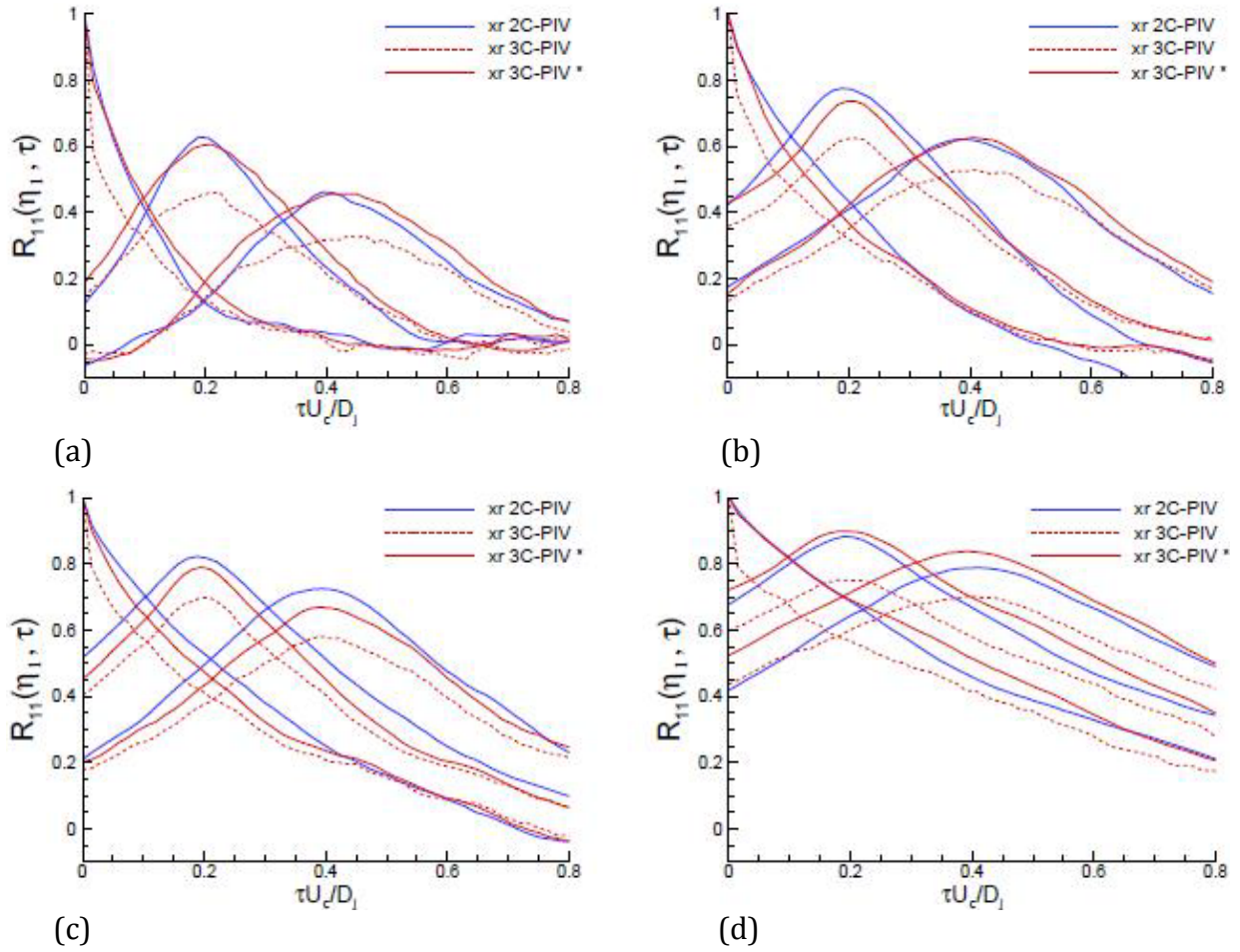
FIGURE 17 (Colour online) R_{11} plots with axial separation - 2C-PIV, 3C-PIV and 3C-PIV* results x/D_j = (a) 1.64, (b) 4.0, (c) 6.5, (d) 10.0
