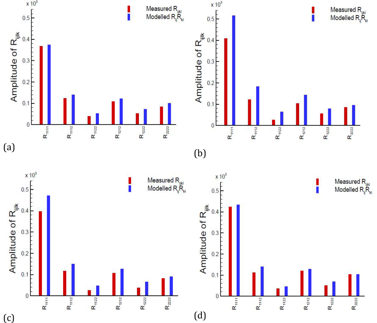
FIGURE 30 (colour online) Comparison between measured and quasi-normal approximation of R_{ij,kl} in x-r plane shear layer: x/D_j = (a) 1.5, (b) 4.0, (c) 6.5, (d) 10.0
