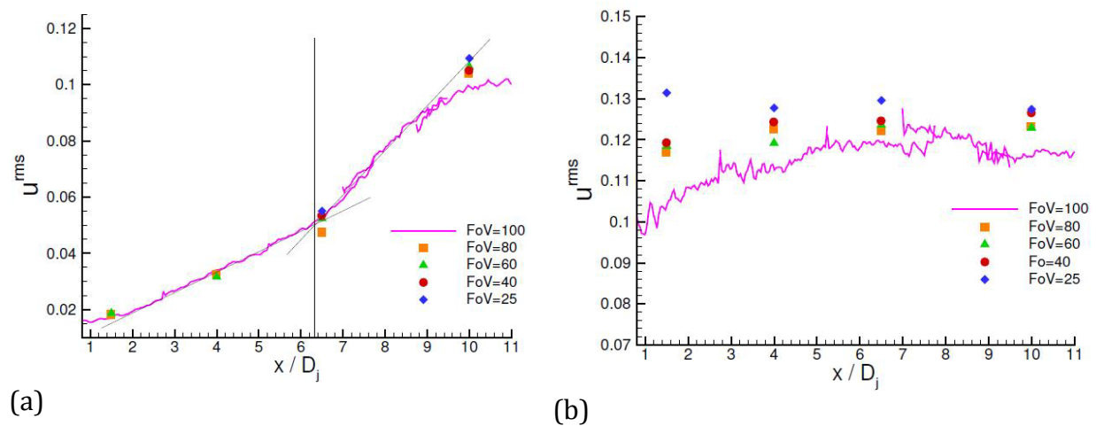
FIGURE 6 (Colour online) Axial development of u_{\text{rms}} for (a) jet centreline and (b) jet lipline
