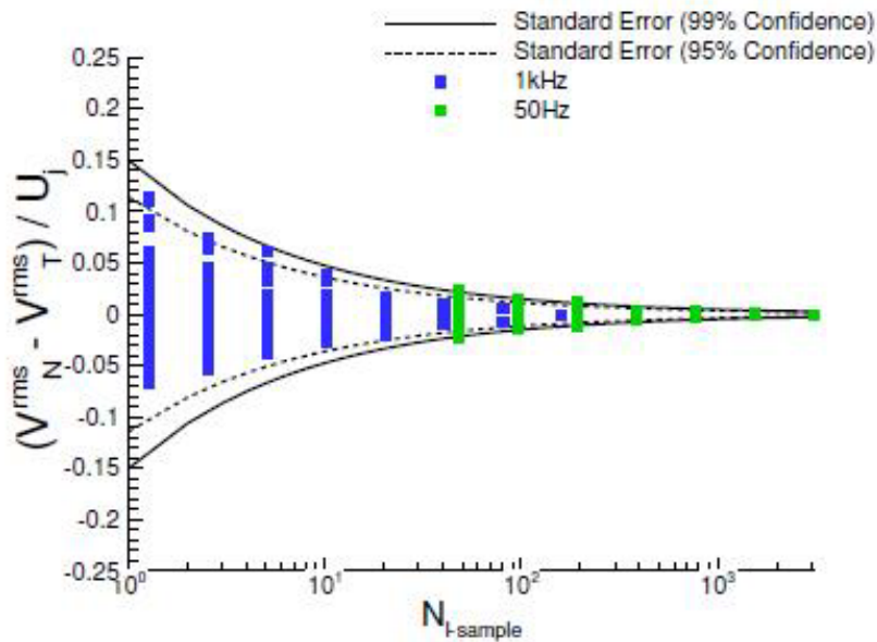
FIGURE 7 (Colour online) Statistical sampling check: v_{rms} at x/D_j = 10.0 , r/D_j = 0.0
