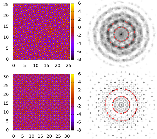
FIG. 13. (Color online) The left panels show plots of \ln[\rho(\mathbf{r})R^2] in the (x/R, y/R) plane obtained from DFT for (a, \rho_0 R^2) = (0.8, 3.5) . The right panels are the corresponding Fourier transforms. The latter exhibit 12-fold symmetry, which is indicative of QC ordering. The top density profile is obtained from random initial conditions, while the lower profile was formed starting from an initial density profile having QC symmetry.
