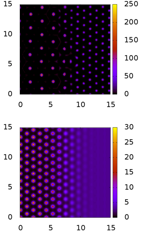
FIG. 2. (Color online) The top panel shows the density profile in the (x/R, y/R) plane near an interface between coexisting crystal A and crystal B phases, for a = 0.75 . Because the lattice spacings of the two crystal structures are not commensurate, defects along the interface are necessarily present. The bottom panel shows the density profile between the uniform liquid and the [1, 1] interface of the crystal B phase, for a = 0.5 .
