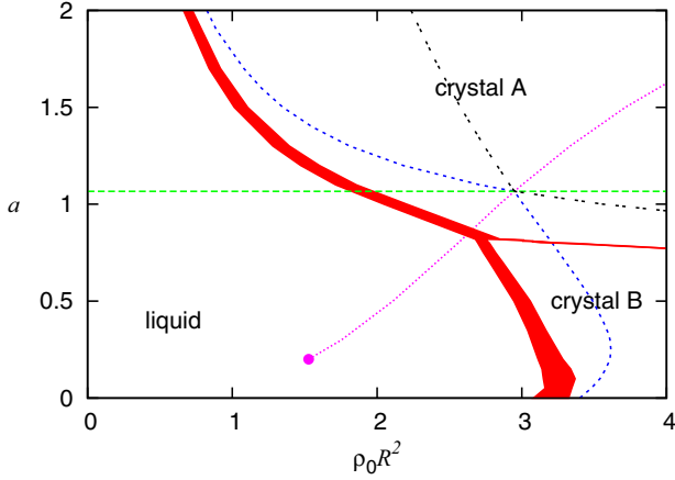
FIG. 1. (Color online) Phase diagram in the (a, \rho_0 R^2) plane, where \rho_0 is the average density. The system exhibits three phases: a liquid and two crystalline phases. Crystal A is hexagonal, with a large lattice spacing, while crystal B, which is also hexagonal, has a smaller lattice spacing. The short-dashed blue line is the linear instability threshold (spinodal) for the uniform liquid. The long-dashed green horizontal line is where the two principal peaks in the static structure factor S(k) have the same height, while the pink dotted line terminating in a circle is the locus where the two peaks in the dispersion relation \omega(k) have equal height. The circle marks the point where the smaller k peak disappears.
