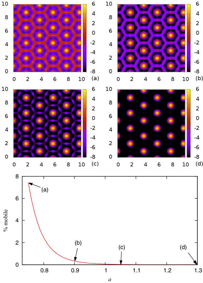
FIG. 9. (Color online) (a)–(d) Plots of \ln[\rho(r)R^2] in the crystal A phase in the (x/R, y/R) plane for fixed \beta\mu = 39 at the state points: (a) (a, \rho_0 R^2) = (0.75, 4.1) , (b) (0.9, 3.8) , (c) (1.05, 3.5) , and (d) (1.3, 3.1) . The bottom figure shows a plot of the fraction of mobile particles that are in the liquid part of the density surrounding the density peaks. For a < 0.75 crystal A is no longer the thermodynamic equilibrium crystal structure and is replaced by crystal B.
