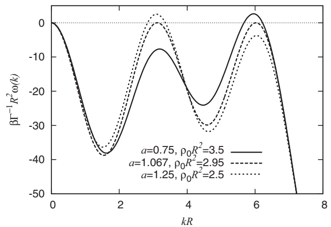
FIG. 6. Dispersion relation \omega(k) at a series of points along a diagonal path in the phase diagram passing through the point at \rho_0 R^2 = 2.95 and a = 1.067 at which the two modes k_1 R = 3.12 and k_2 R = 6.03 are simultaneously marginally unstable. Note that k_2/k_1 = 1.932 .
