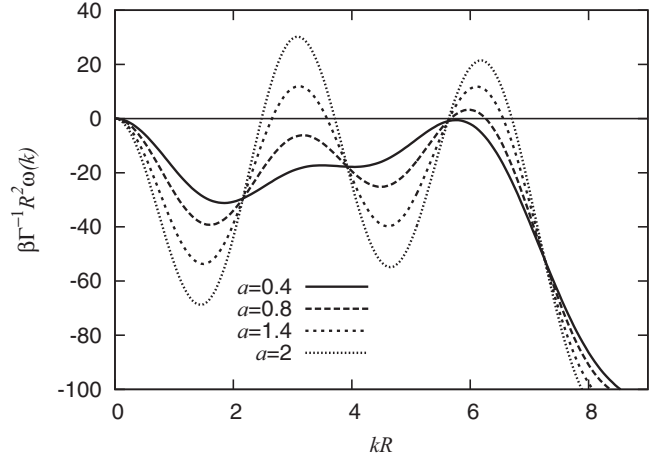
FIG. 5. Dispersion relation \omega(k) for fixed \rho_0 R^2 = 3.5 and various values of a , as indicated in the key.
