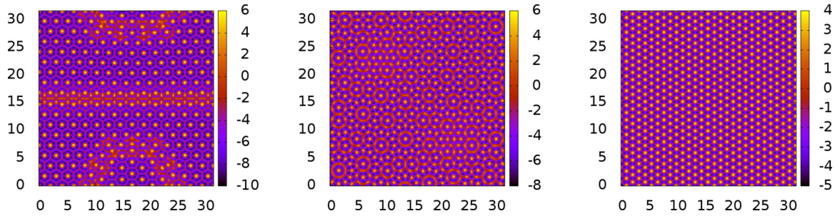
FIG. 15. (Color online) Plots of \ln[\rho(\mathbf{r})R^2] in the (x/R, y/R) plane for density profiles obtained when starting from the perfect QC displayed on the bottom left of Fig. 13, which has R_s/R = 1.855 , and then following the solution as R_s is varied, for fixed \mu and domain size. When R_s is decreased, the QC remains stable until R_s/R = 1.77 , at which point the QC profile becomes linearly unstable and the Picard iteration then falls on to the crystal A profile (which contains defects), displayed above left. When R_s is instead increased, the perfect QC solutions become unstable at R_s/R = 2.03 , where the iteration switches to a different branch of QC solutions (above middle), before this new QC state becomes unstable at R_s/R = 2.19 and evolves to the crystal B branch of solutions displayed above right.
