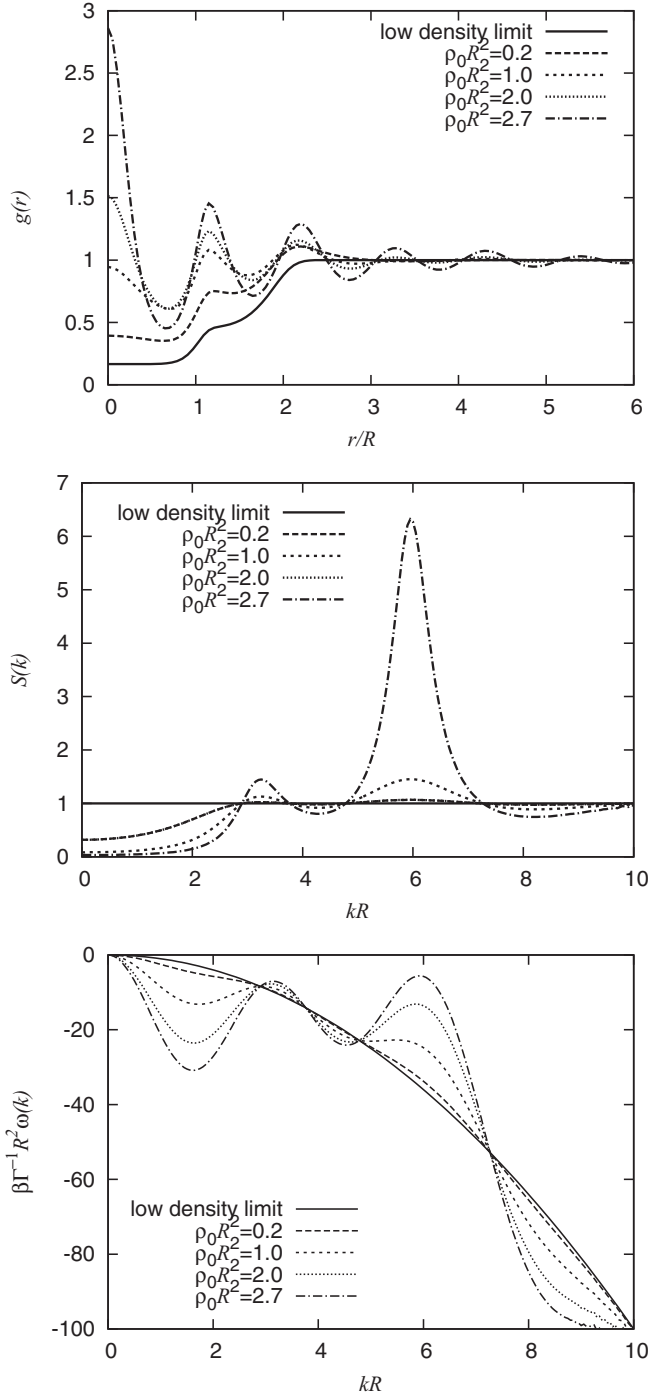
FIG. 3. Correlation functions characterizing the liquid phase for increasing density \rho_0 as indicated in the key, for fixed a = 0.8 . The top panel shows the radial distribution function g(r) , the middle panel the static structure factor S(k) , and the bottom panel the dispersion relation \omega(k) .
