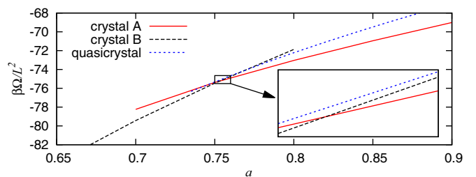
FIG. 14. (Color online) Grand potential density as a function of a for fixed \beta\mu = 39 for the two different crystal structures and also the QC solution displayed in Fig. 13. Near a = 0.75 there is a point where all three have almost the same value of the grand potential, but the QC solution is never the global minimum (see the inset). The crystal A phase is of crystal-liquid type throughout the range of a shown.
