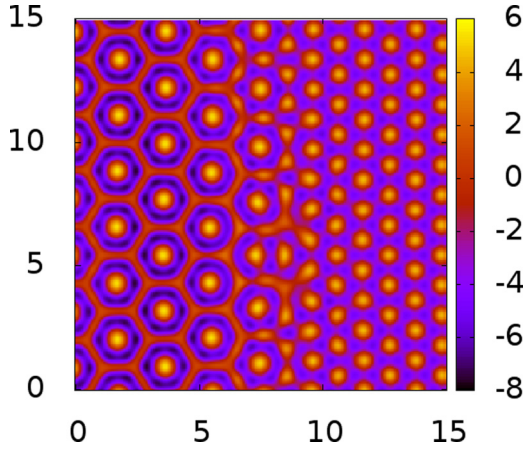
FIG. 7. (Color online) Density profile in the top panel of Fig. 2 displayed in terms of the logarithm of the density \ln[\rho(\mathbf{r})R^2] plotted in the (x/R, y/R) plane. This representation allows one to see the fine structure of the density profile away from the principal peaks. Note in particular the honeycomb structure surrounding each of the peaks in the crystal A phase on the left of the interface.
