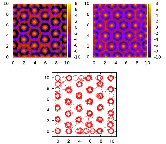
FIG. 8. (Color online) The top panels show \ln[\rho(\mathbf{r})R^2] in the (x/R, y/R) plane for a system of N = 600 particles with (a, \rho_0 R^2) = (0.8, 6) confined in a square region of side L = 10R obtained from BD simulations (top left) and DFT (top right). The system forms crystal A with a density profile consisting of an array of peaks surrounded by a connected network within which the particles are free to move; this is the crystal-liquid state. The bottom panel is a snapshot from the BD simulation where each particle coordinate is plotted as an open circle.
