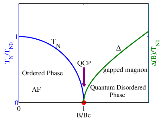
FIG. 1 (color online). Schematic phase diagram for a QPT, showing the Néel temperature and spin gap as functions of magnetic field [14]. For a magnetic QPT, the characteristic energy scales in the quantum disordered (QD) and AF phases are, respectively, the spin gap \Delta and Néel temperature T_N , and both vanish at the QCP.
