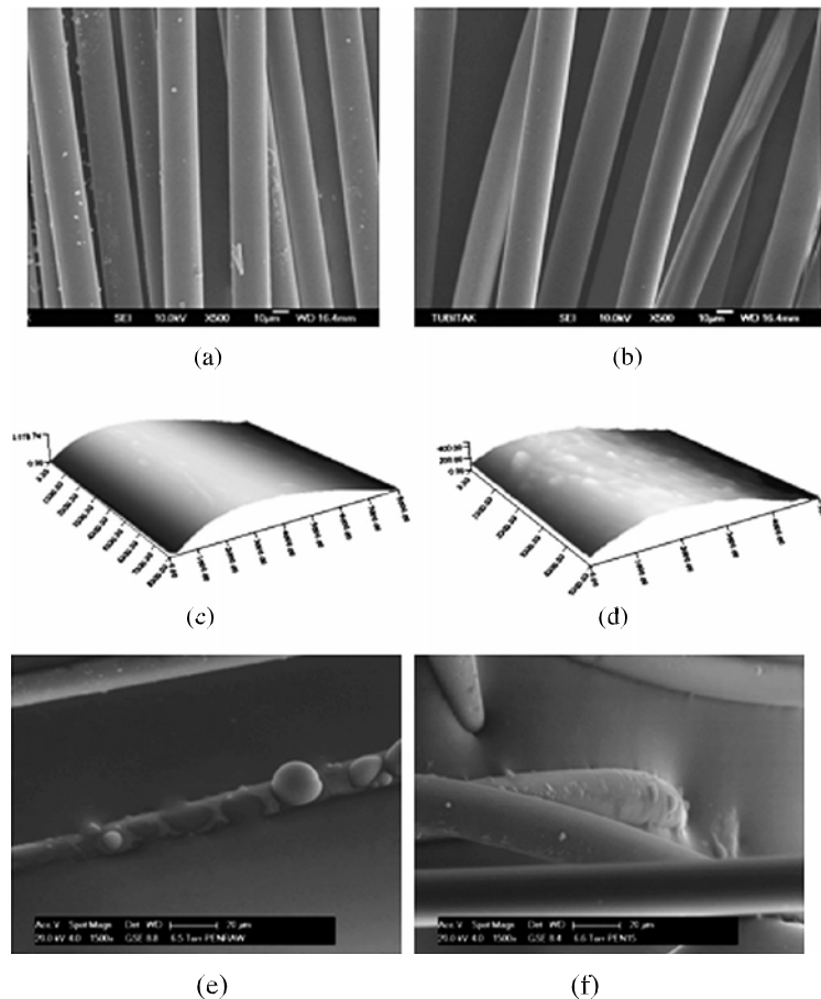
Figure 6. SEM, AFM and ESEM images of PEN fibers respectively: (a) PEN Raw, (b) PEN20, PEN Raw, (d) PEN20, (e) PEN Raw and (f) PEN15.
