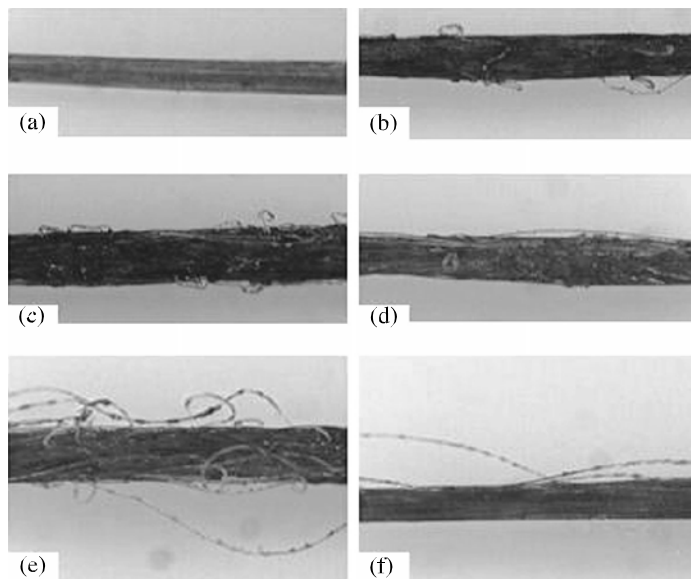
Figure 8. Optical microscopy images of the air-jet textured yarns after dipping process: (a) a typical polyester yarn before air-jet texturing, (b) FDY20, (c) DSPET20, (d) HTPET20, (e) PEN20 and (f) Vectran20.
