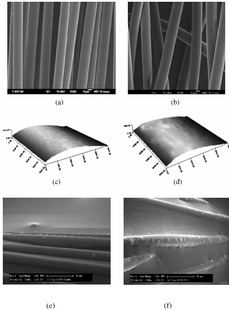
Figure 5. SEM, AFM and ESEM images of HTPET fibers respectively: (a) HTPET Raw, (b) HTPET20, (c) HTPET Raw, (d) HTPET20, (e) HTPET Raw and (f) HTPET15.
