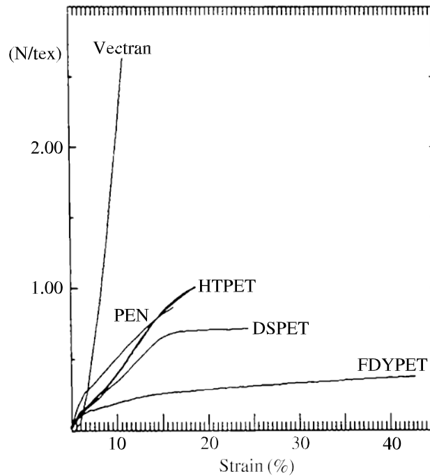
Figure 1. Stress-strain curves of single fibers.
