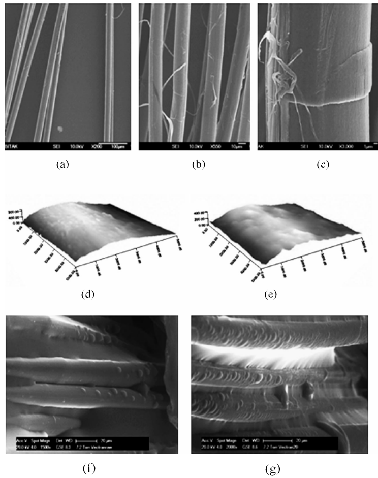
Figure 7. SEM, AFM and ESEM images of Vectran fibers respectively: (a) Vectran Raw, (b) Vectran20, (c) Vectran20, (d) Vectran Raw, (e) Vectran 20, (f) Vectran Raw and (g) Vectran15.
