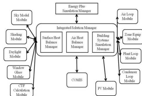
Figure 6 Energy plus modules
