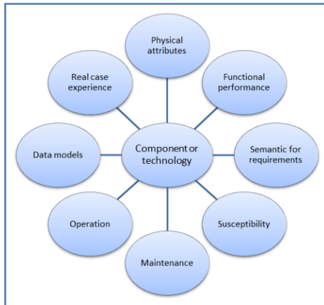
Figure 4 Database schema
