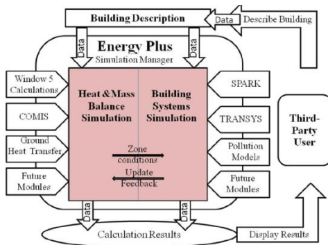
Figure 5 Energy plus flow chart
