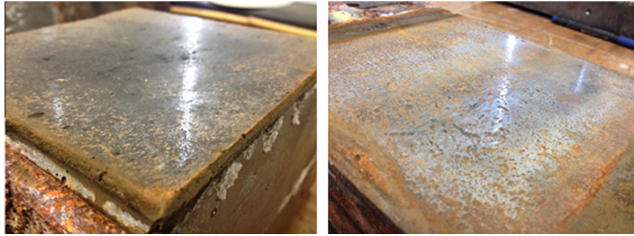
Fig. 5. Post-test grout (left) and steel (right) surfaces of a wet sample.
