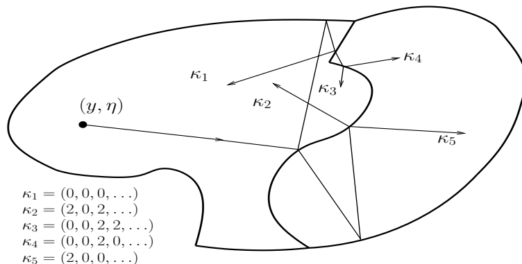
FIGURE 3. Ray-splitting trajectories
