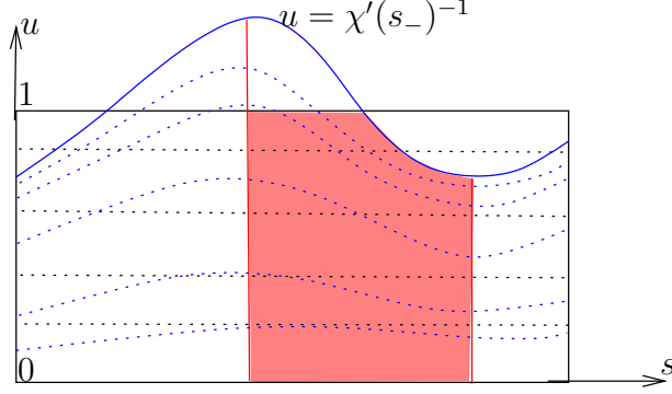
FIGURE 4. Poincaré section.
