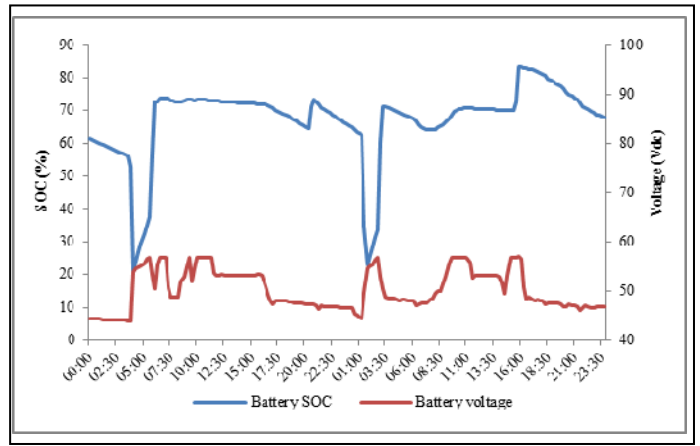
Fig. 6. Battery state of charge (SOC) and voltage on 17-18/2011 at SK Poring.
