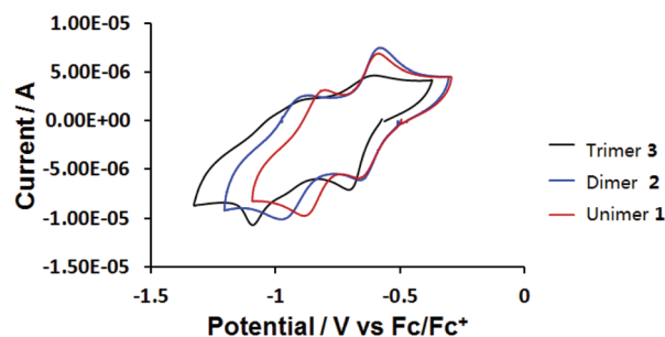
Fig. 4 Cyclic voltammograms of 0.2 mM compounds 1 , 2 and 3 at a glassy carbon disc ( d = 2 mm) electrode in anhydrous DMF at v = 500 mV \text{s}^{-1} .
