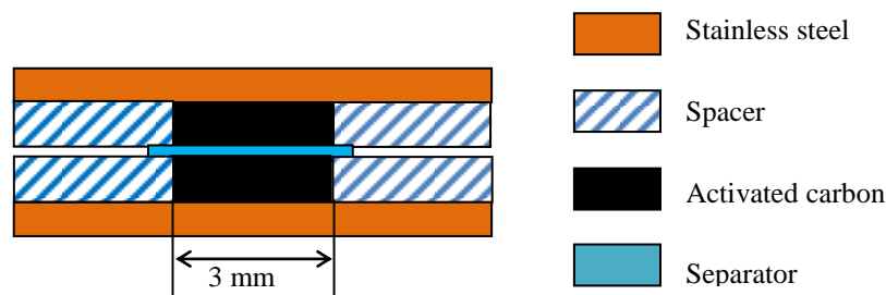
Figure 1. Schematic diagram of the strip supercapacitor.
